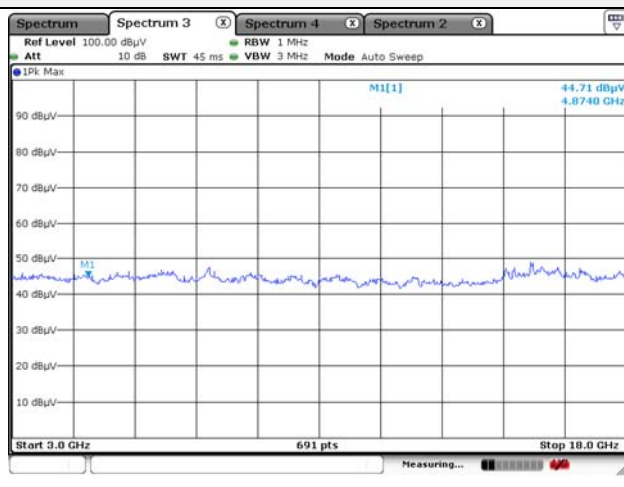
Vertical // Peak for 3 GHz to 18 GHz
