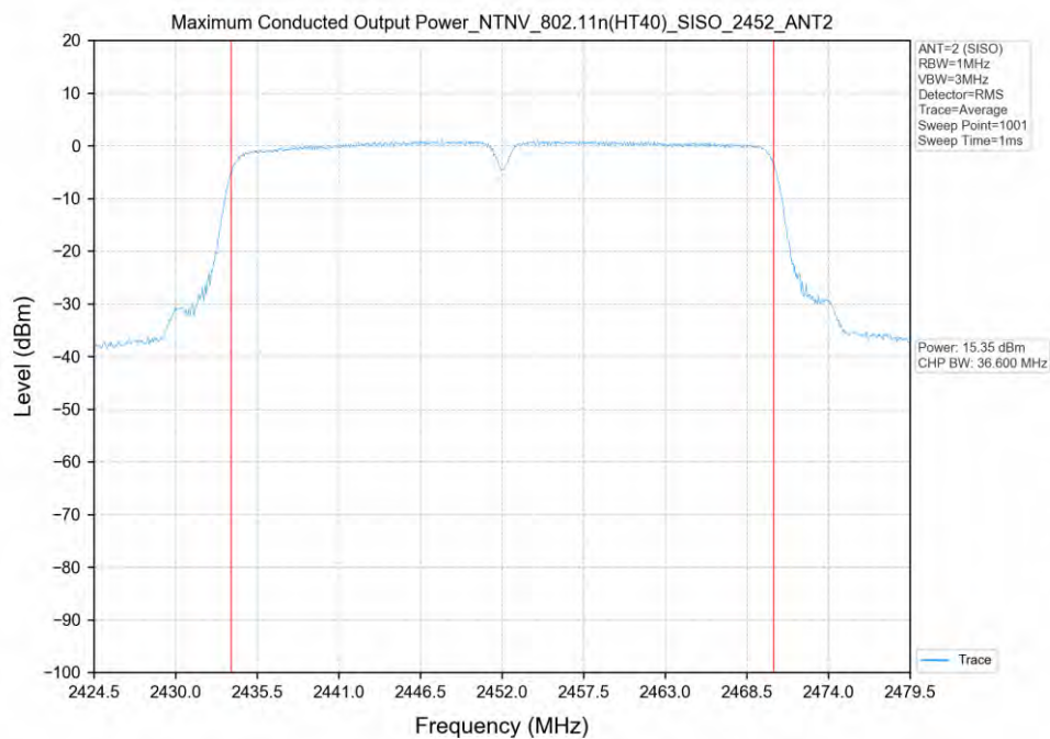
802.11n(HT40) 2452MHz SISO ANT2
