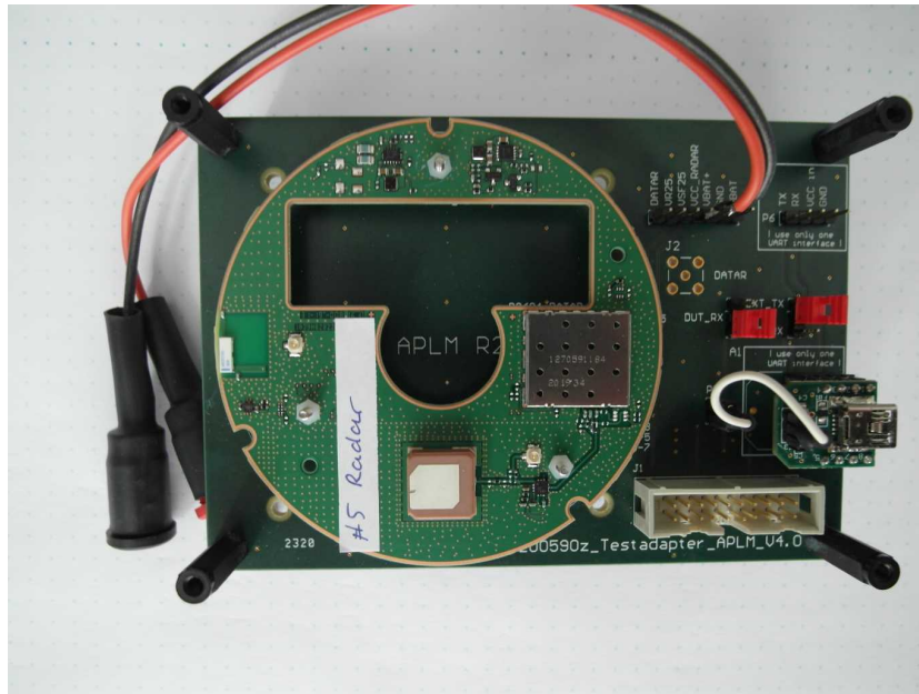
Photo 9 DUT Programming Board (JIG) + DUT PCB
