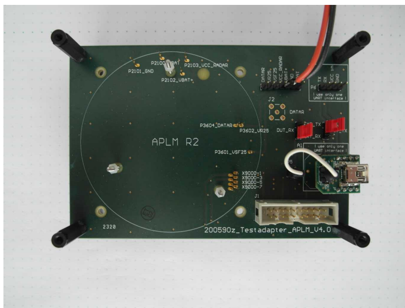
Photo 8 DUT Programming Board (JIG) Top
