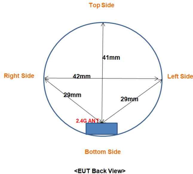
Fig 7.1 Block Diagram for EUT Antenna Position
