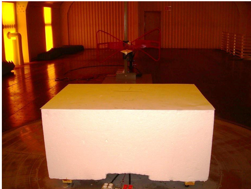
Photograph 6: Test Setup for Emission from 30 MHz to 1000 MHz
