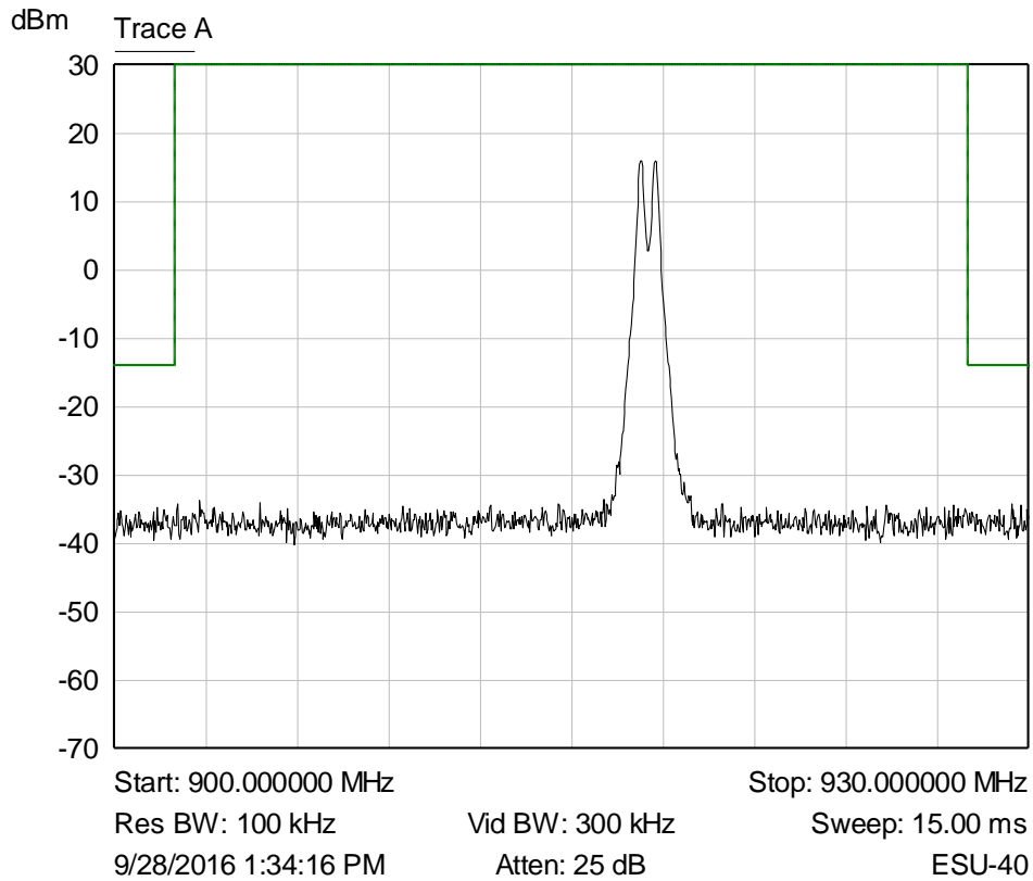
Graph 3: Operating Band Plot
