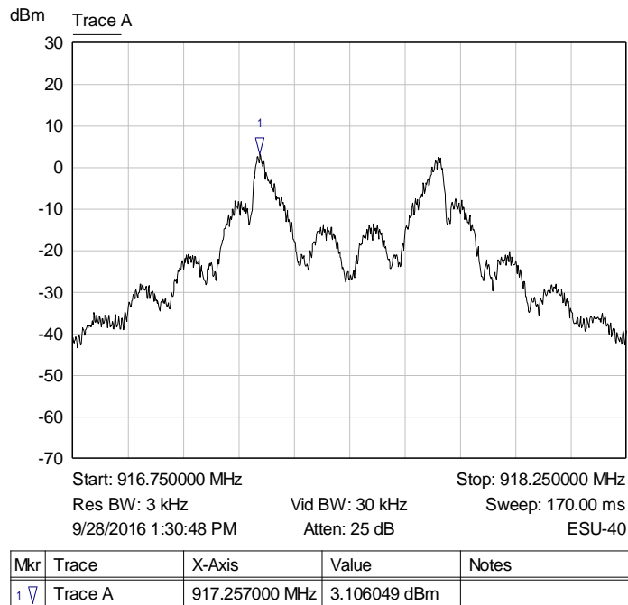
Graph 4: 3 kHz PSD Plot
