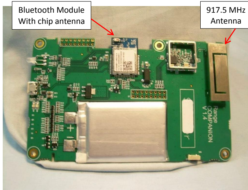
Photograph 1 – View of the Component Side of the PCB
