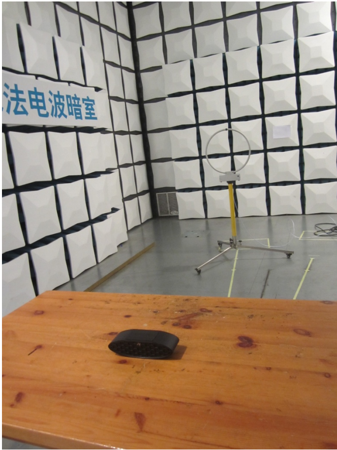
Radiated Emission
