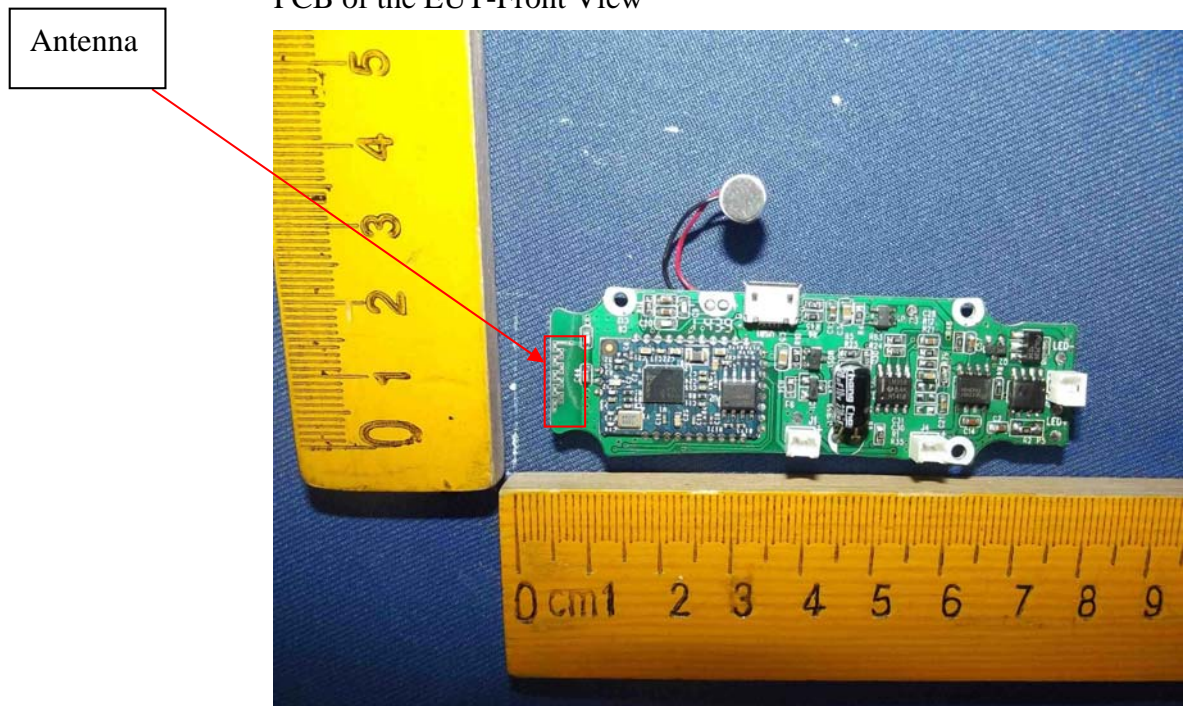
Figure 12 PCB of the EUT-Front View
