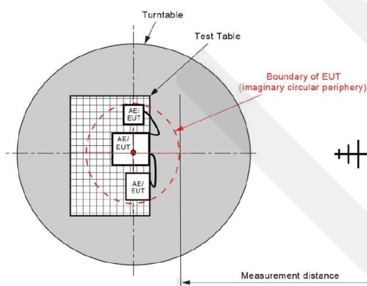
Figure C.1 – Measurement distance
