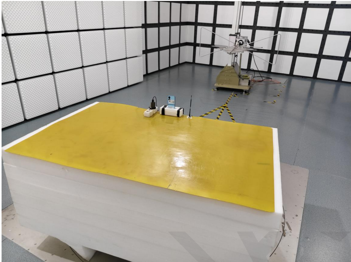
Radiated Spurious Emissions Test View (Below 1GHz)
