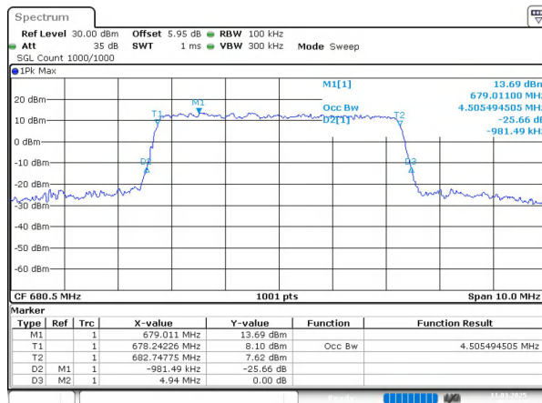
n71 SCS=15kHz CP_QPSK BW=5MHz Channel=136100 RB=25@0
