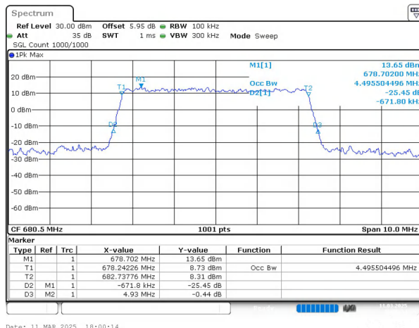
n71 SCS=15kHz CP_64QAM BW=5MHz Channel=136100 RB=25@0
