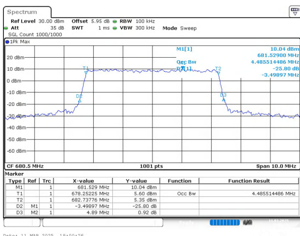
n71 SCS=15kHz CP_256QAM BW=5MHz Channel=136100 RB=25@0
