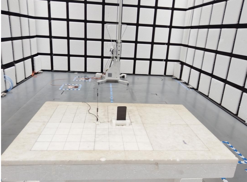
Radiated spurious emission Test Setup-2(Above 1GHz)
