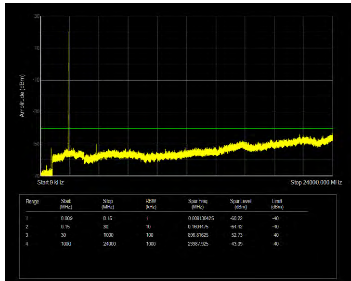
Band30 QPSK BW=5MHz Channel=27735 RB Size=1 Position=#0
