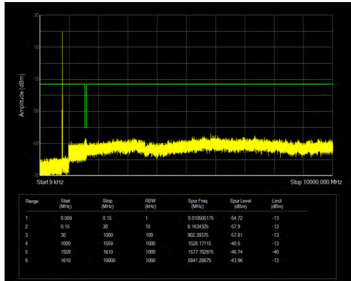
Band14 QPSK BW=10MHz Channel=23330 RB Size=50 Position=#0
