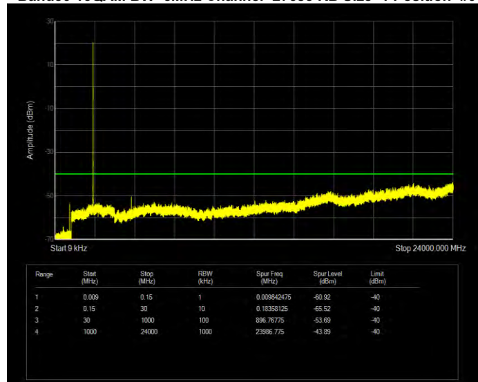
Band30 16QAM BW=10MHz Channel=27710 RB Size=1 Position=#0
