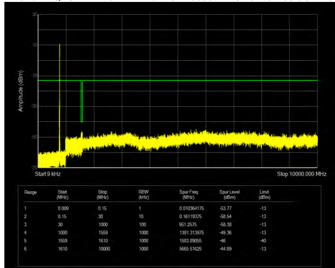
Band14 QPSK BW=5MHz Channel=23330 RB Size=25 Position=#0
