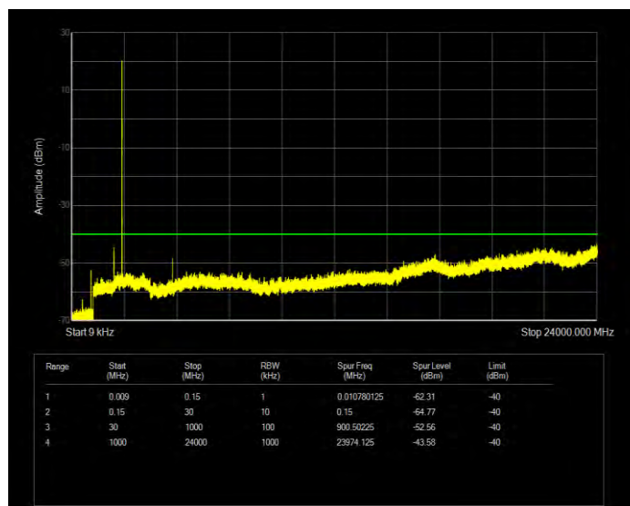
Band30 QPSK BW=10MHz Channel=27710 RB Size=1 Position=#0
