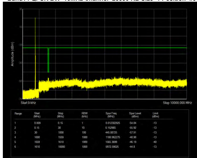
Band14 QPSK BW=5MHz Channel=23305 RB Size=1 Position=#0
