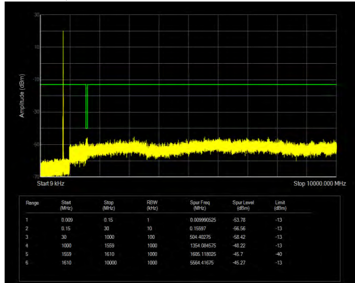
Band14 QPSK BW=5MHz Channel=23355 RB Size=1 Position=#0
