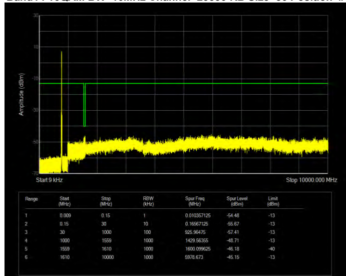
Band14 16QAM BW=5MHz Channel=23305 RB Size=25 Position=#0
