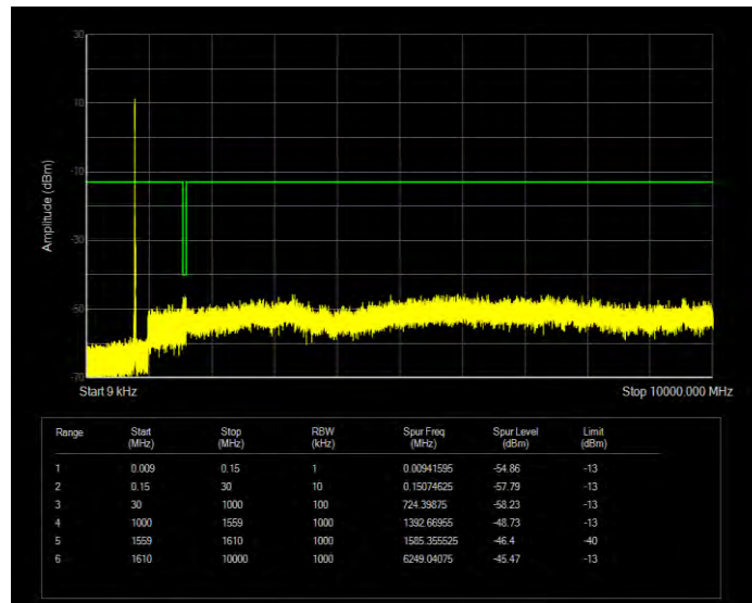
Band14 16QAM BW=5MHz Channel=23355 RB Size=1 Position=#0
