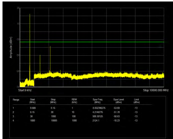
Band30 16QAM BW=5MHz Channel=27685 RB Size=1 Position=#0
