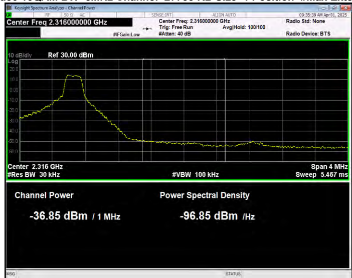
Band30 16QAM BW=5MHz Channel=27735 RB Size=1 Position=#0 Normal
