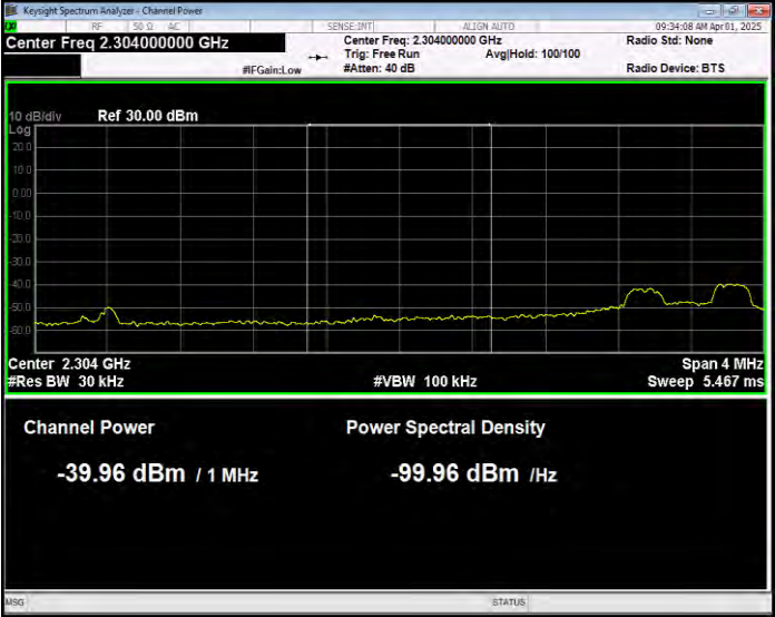
Band30 16QAM BW=5MHz Channel=27685 RB Size=1 Position=#Max Normal
