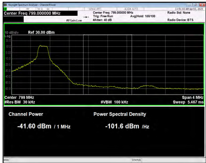
Band14 QPSK BW=5MHz Channel=23355 RB Size=25 Position=#0 Extended
