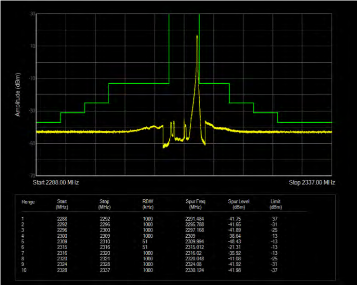
Band30 16QAM BW=5MHz Channel=27735 RB Size=25 Position=#0 Extended
