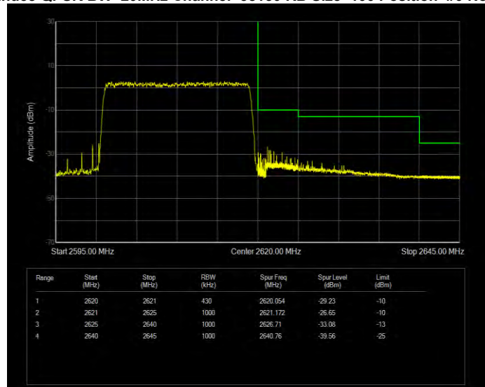
Band38 QPSK BW=20MHz Channel=38150 RB Size=1 Position=#Max Normal
