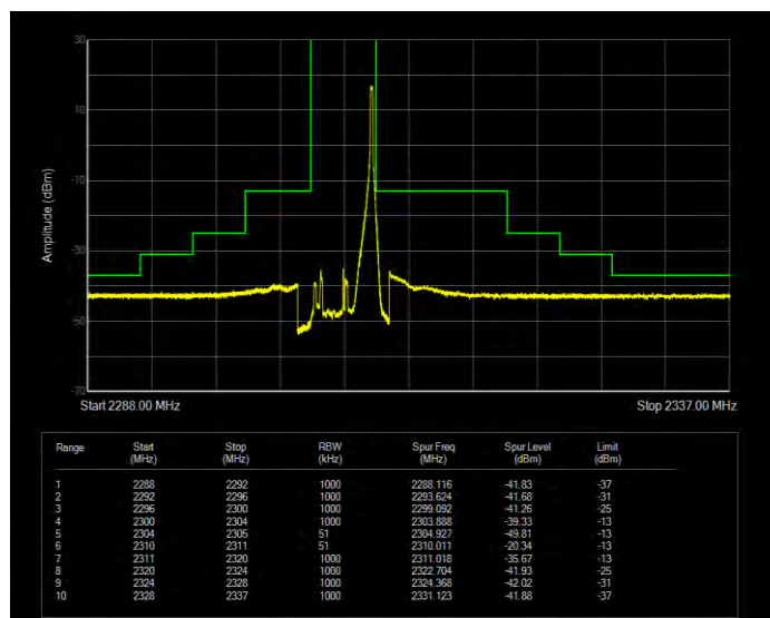
Band30 QPSK BW=5MHz Channel=27685 RB Size=25 Position=#0 Extended
