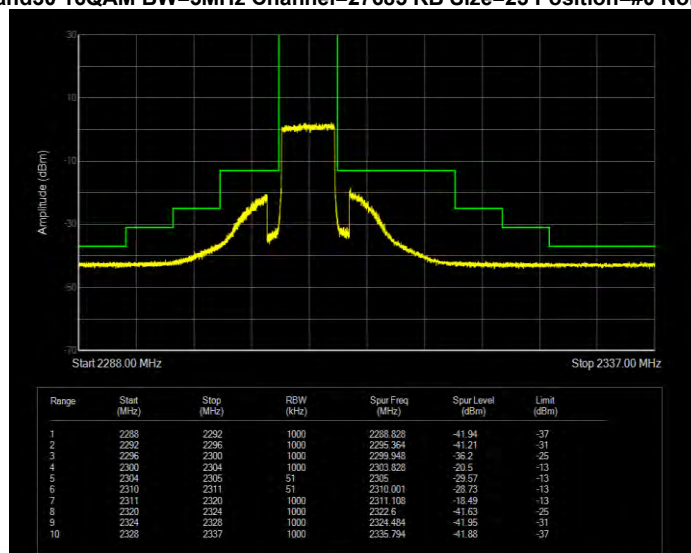
Band30 16QAM BW=5MHz Channel=27685 RB Size=25 Position=#0 Extended
