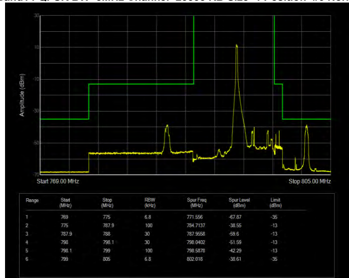
Band14 QPSK BW=5MHz Channel=23355 RB Size=1 Position=#Max Normal
