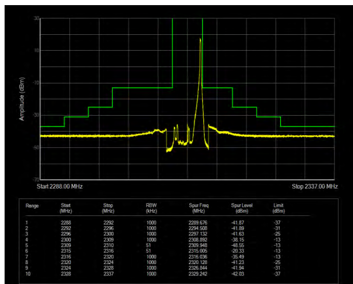
Band30 QPSK BW=5MHz Channel=27735 RB Size=25 Position=#0 Normal
