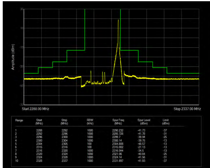
Band30 16QAM BW=10MHz Channel=27710 RB Size=50 Position=#0 Extended
