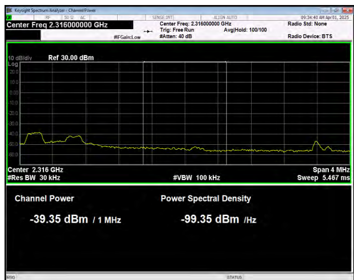
Band30 QPSK BW=5MHz Channel=27735 RB Size=1 Position=#Max Extended
