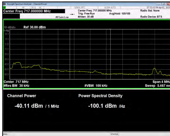
Band17 QPSK BW=5MHz Channel=23825 RB Size=1 Position=#Max Extended
