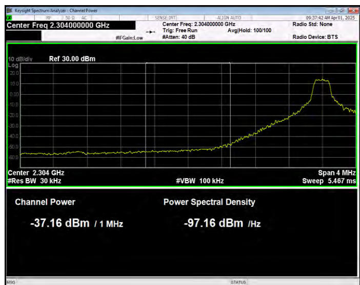
Band30 16QAM BW=10MHz Channel=27710 RB Size=1 Position=#0 Normal
