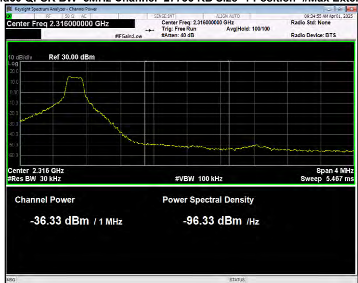
Band30 QPSK BW=5MHz Channel=27735 RB Size=1 Position=#0 Normal
