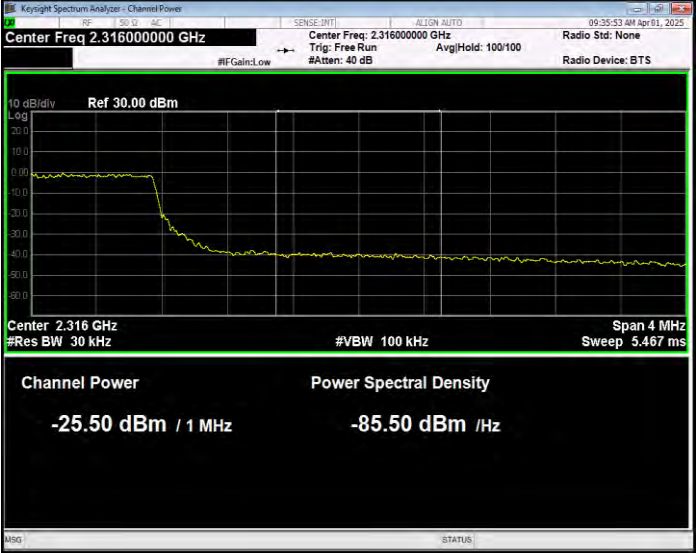
Band30 QPSK BW=10MHz Channel=27710 RB Size=1 Position=#0 Extended
