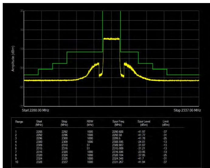
Band30 QPSK BW=10MHz Channel=27710 RB Size=1 Position=#0 Normal
