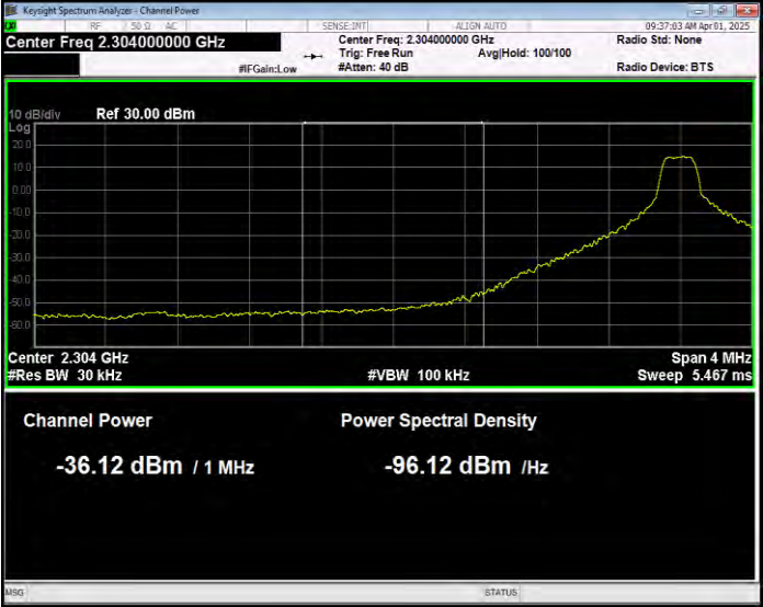
Band30 16QAM BW=5MHz Channel=27735 RB Size=25 Position=#0 Normal
