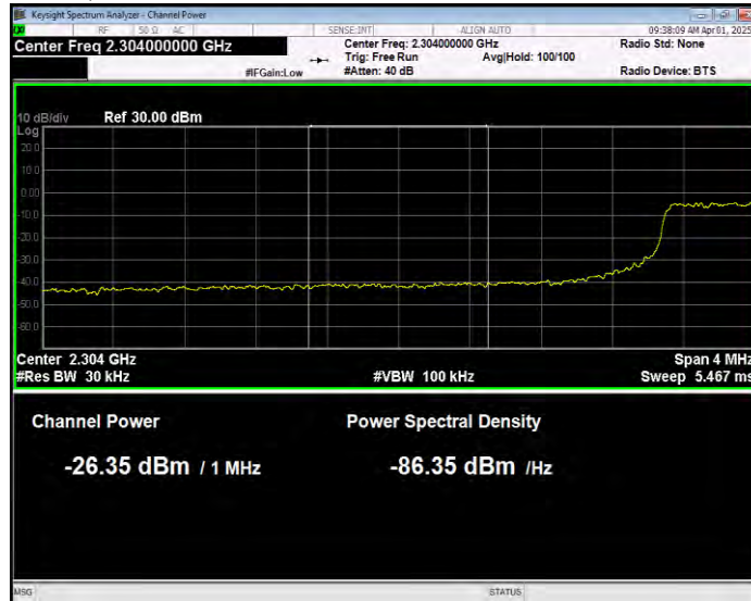
Band30 16QAM BW=10MHz Channel=27710 RB Size=50 Position=#0 Normal
