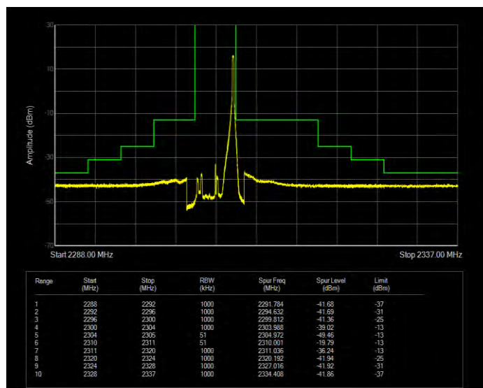
Band30 16QAM BW=5MHz Channel=27685 RB Size=25 Position=#0 Normal
