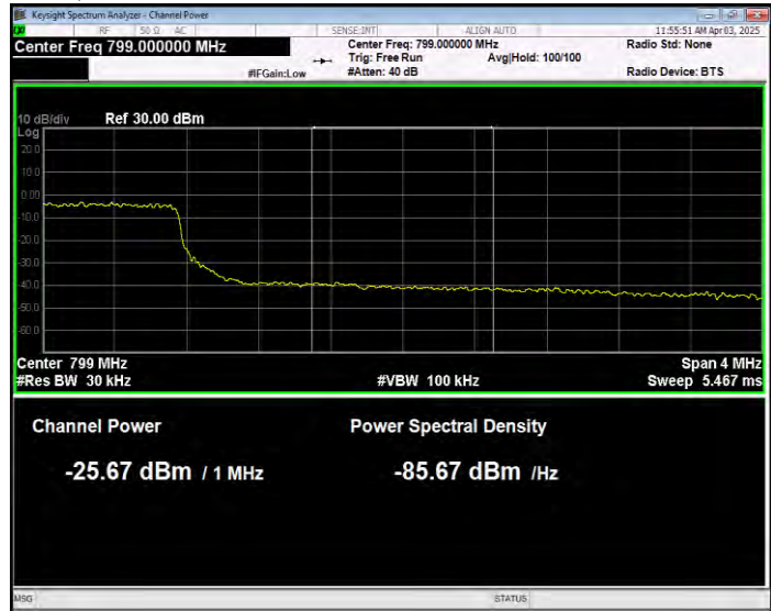
Band14 QPSK BW=5MHz Channel=23355 RB Size=25 Position=#0 Normal
