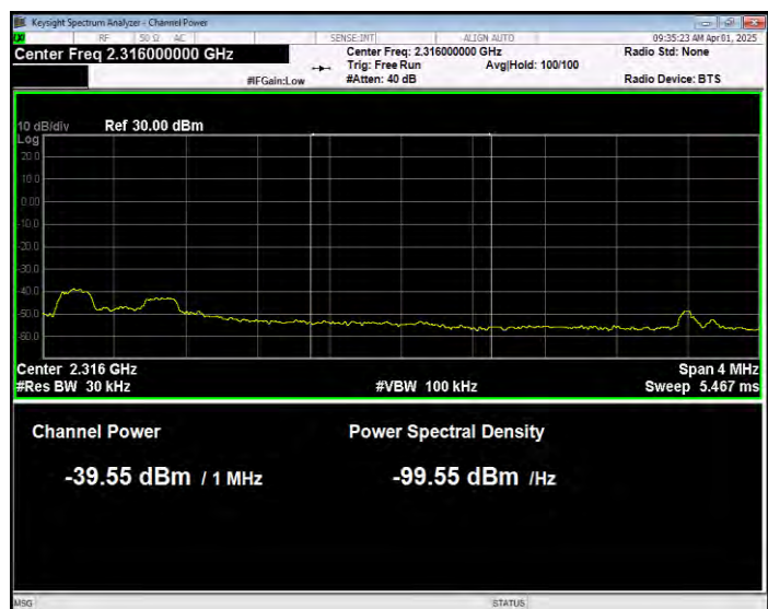
Band30 16QAM BW=5MHz Channel=27735 RB Size=1 Position=#Max Extended
