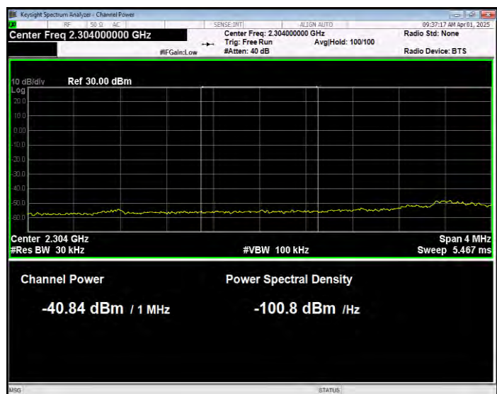
Band30 QPSK BW=10MHz Channel=27710 RB Size=50 Position=#0 Extended
