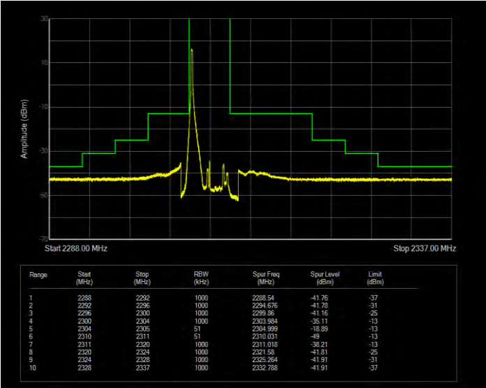
Band30 16QAM BW=5MHz Channel=27685 RB Size=1 Position=#0 Extended
