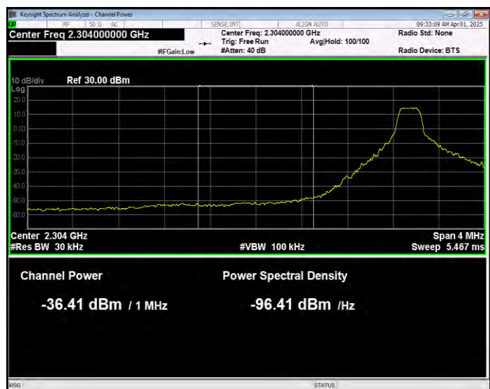
Band30 QPSK BW=5MHz Channel=27685 RB Size=1 Position=#Max Extended
