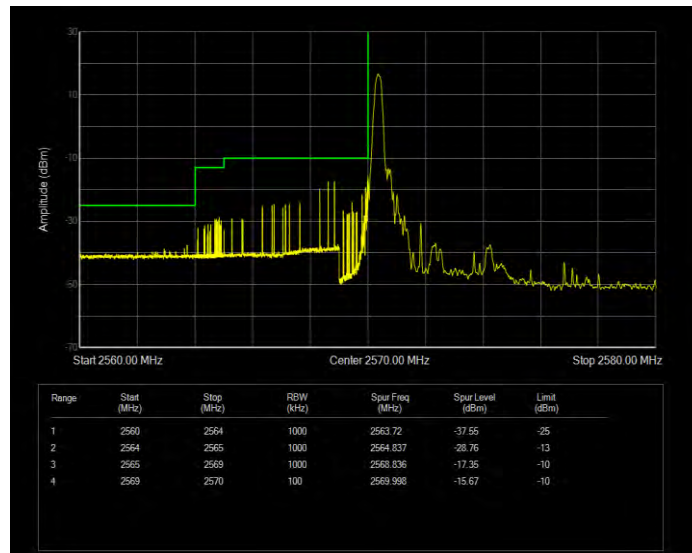
Band38 QPSK BW=5MHz Channel=37775 RB Size=1 Position=#Max Normal
