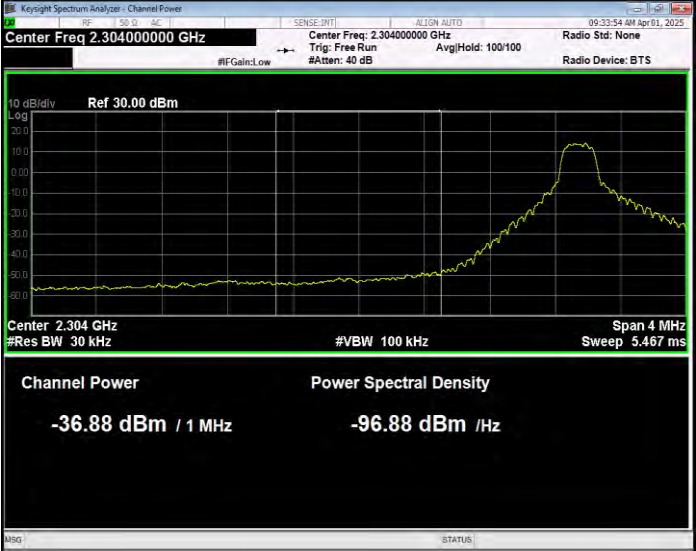
Band30 16QAM BW=5MHz Channel=27685 RB Size=1 Position=#Max Extended
