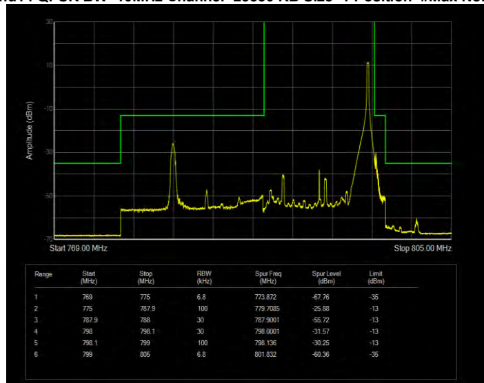
Band14 QPSK BW=10MHz Channel=23330 RB Size=1 Position=#Max Extended
