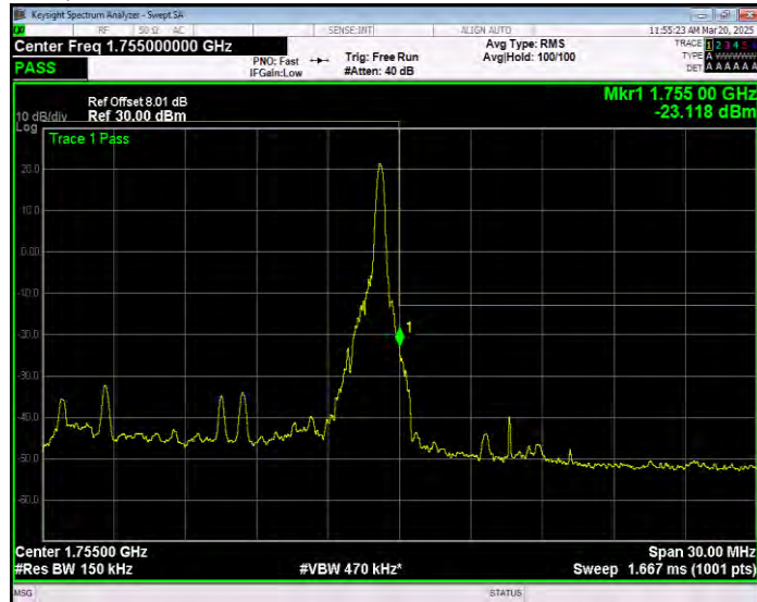
Band4 QPSK BW=15MHz Channel=20325 RB Size=75 Position=#0 Normal
