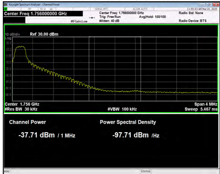
Band4 16QAM BW=15MHz Channel=20325 RB Size=75 Position=#0 Extended
