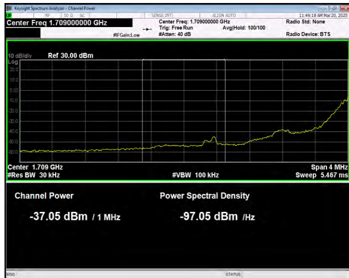
Band4 16QAM BW=1.4MHz Channel=19957 RB Size=6 Position=#0 Normal
