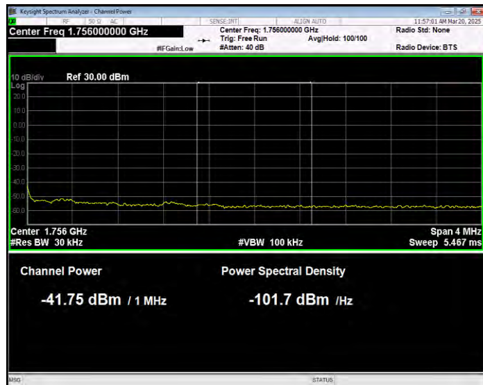
Band4 16QAM BW=20MHz Channel=20300 RB Size=1 Position=#Max Extended
