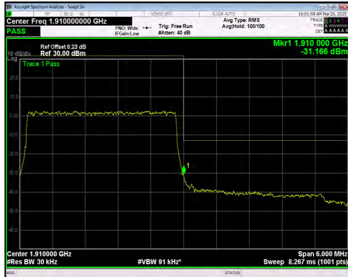
Band2 QPSK BW=3MHz Channel=19185 RB Size=1 Position=#Max Normal
