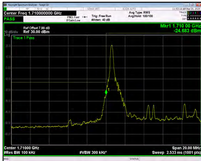
Band4 QPSK BW=10MHz Channel=20000 RB Size=1 Position=#0 Extended
