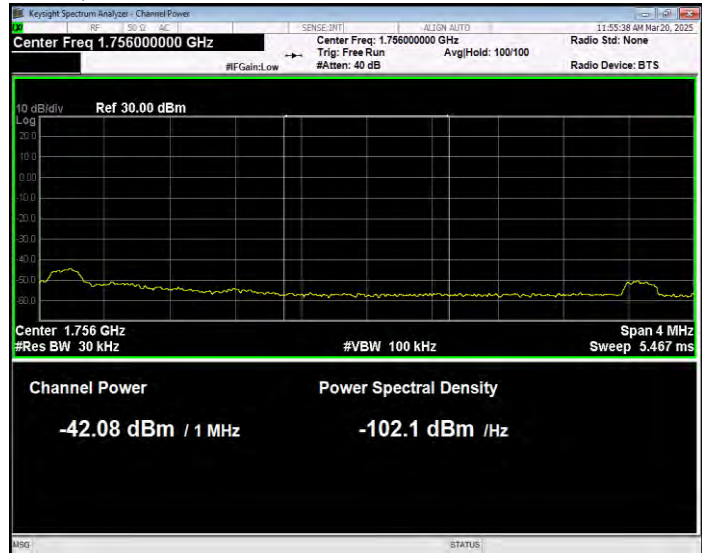
Band4 16QAM BW=15MHz Channel=20325 RB Size=1 Position=#Max Extended
