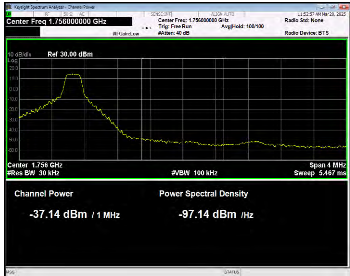
Band4 16QAM BW=5MHz Channel=20375 RB Size=1 Position=#Max Normal
