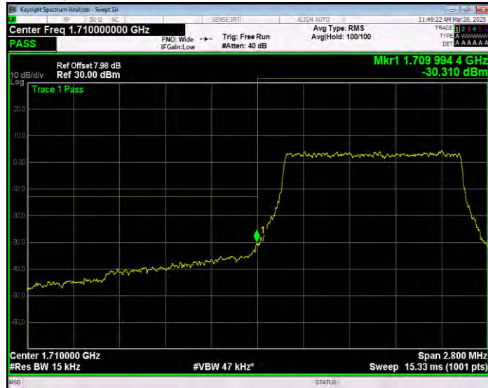
Band4 16QAM BW=1.4MHz Channel=19957 RB Size=6 Position=#0 Extended
