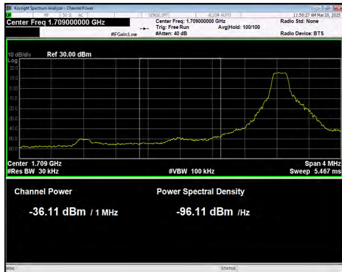
Band4 QPSK BW=3MHz Channel=19965 RB Size=1 Position=#Max Extended
