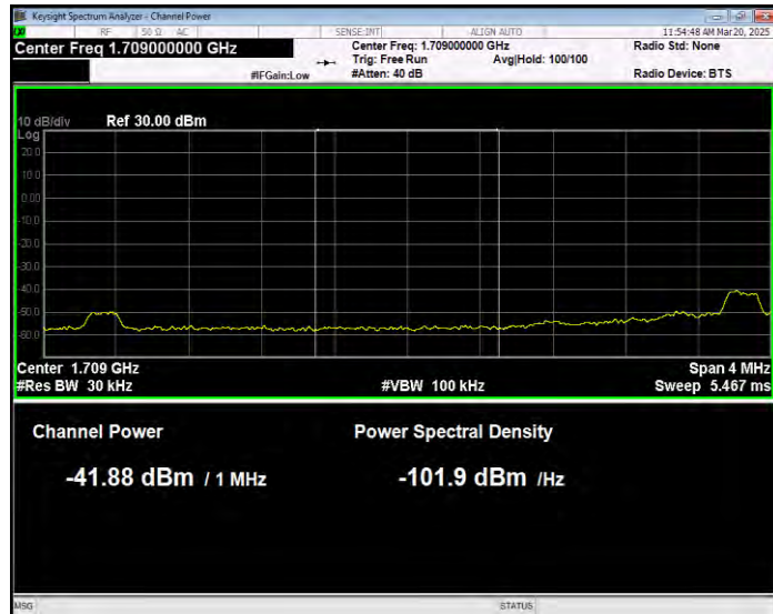
Band4 QPSK BW=15MHz Channel=20025 RB Size=75 Position=#0 Extended
