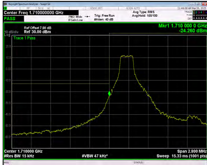
Band4 16QAM BW=1.4MHz Channel=19957 RB Size=1 Position=#Max Normal
