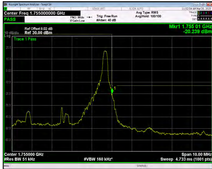
Band4 16QAM BW=5MHz Channel=20375 RB Size=25 Position=#0 Extended
