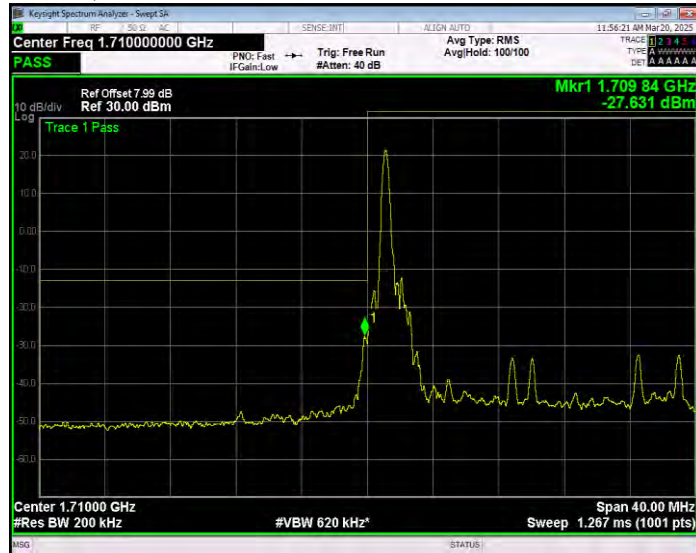
Band4 16QAM BW=20MHz Channel=20050 RB Size=1 Position=#Max Normal
