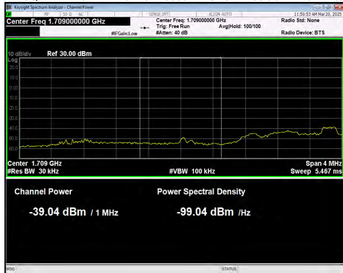
Band4 16QAM BW=3MHz Channel=19965 RB Size=15 Position=#0 Extended
