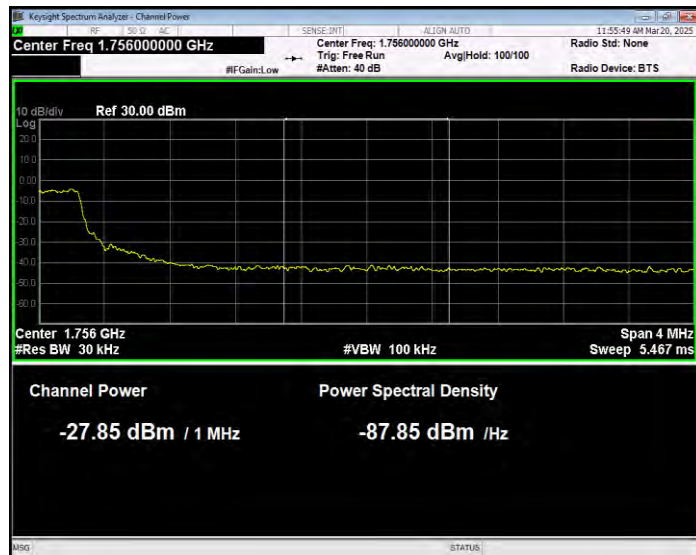
Band4 16QAM BW=15MHz Channel=20325 RB Size=1 Position=#Max Normal
