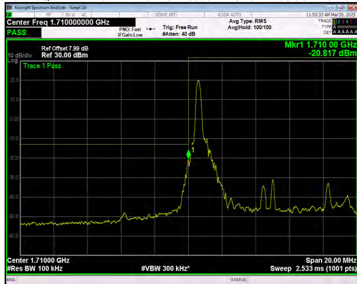
Band4 16QAM BW=10MHz Channel=20000 RB Size=1 Position=#Max Normal
