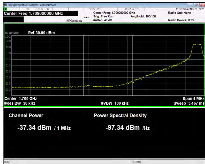
Band4 16QAM BW=15MHz Channel=20025 RB Size=1 Position=#0 Normal
