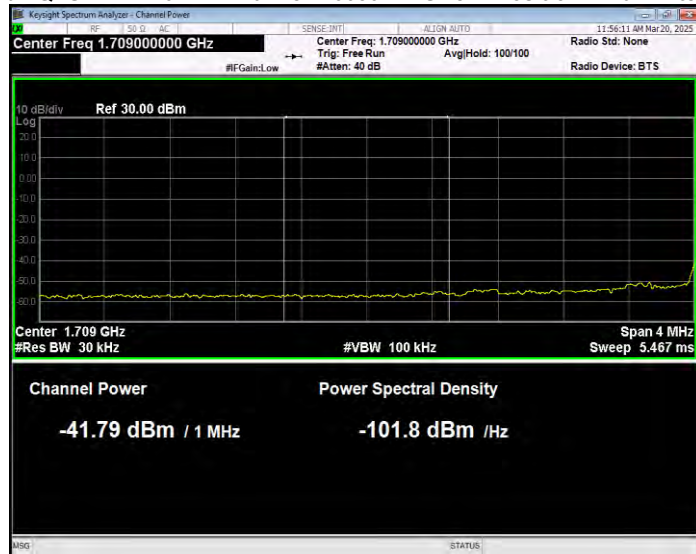
Band4 QPSK BW=20MHz Channel=20050 RB Size=100 Position=#0 Extended
