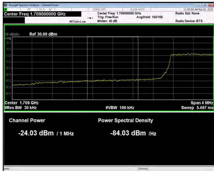
Band4 16QAM BW=3MHz Channel=19965 RB Size=1 Position=#Max Normal
