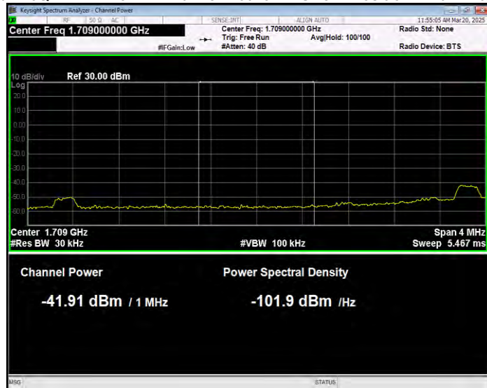
Band4 16QAM BW=15MHz Channel=20025 RB Size=1 Position=#Max Normal
