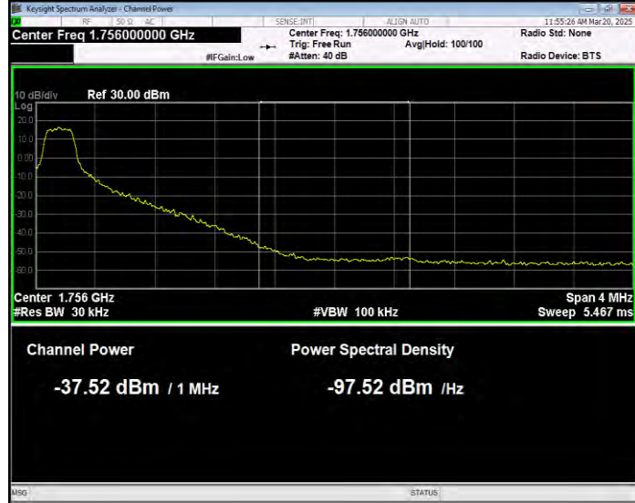
Band4 QPSK BW=15MHz Channel=20325 RB Size=75 Position=#0 Extended
