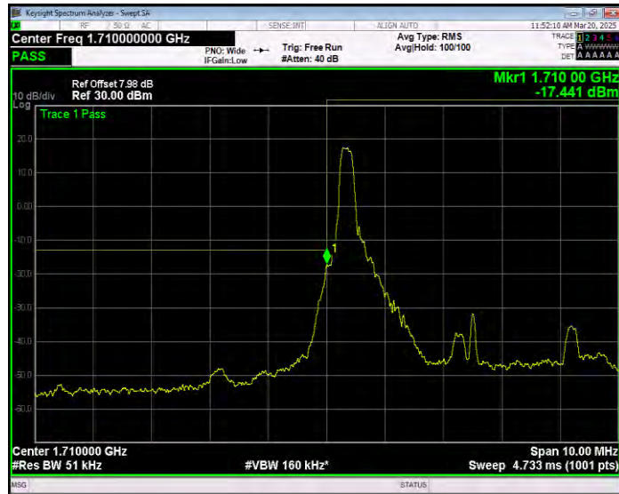
Band4 16QAM BW=5MHz Channel=19975 RB Size=1 Position=#0 Extended
