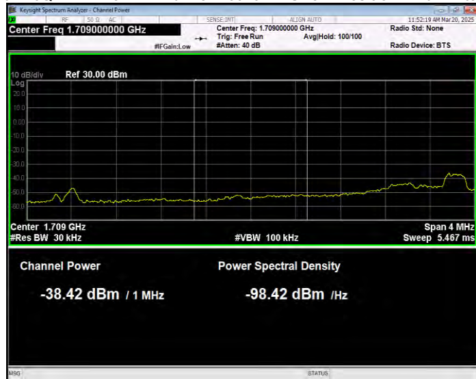
Band4 16QAM BW=5MHz Channel=19975 RB Size=1 Position=#Max Normal
