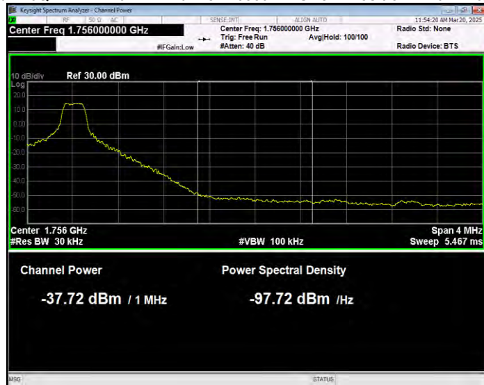
Band4 16QAM BW=10MHz Channel=20350 RB Size=1 Position=#Max Normal
