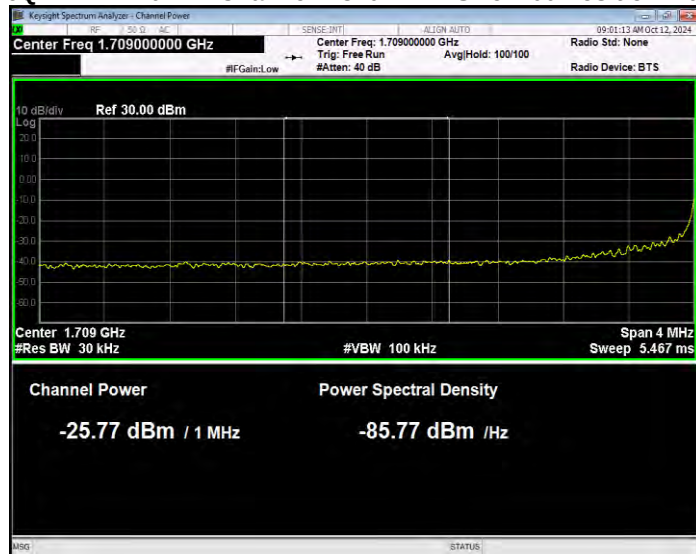
Band66 16QAM BW=20MHz Channel=132072 RB Size=100 Position=#0 Normal
