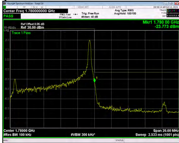
Band66 QPSK BW=10MHz Channel=132622 RB Size=50 Position=#0 Extended
