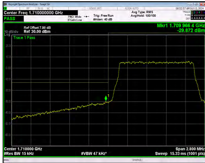
Band66 QPSK BW=1.4MHz Channel=132665 RB Size=1 Position=#0 Extended
