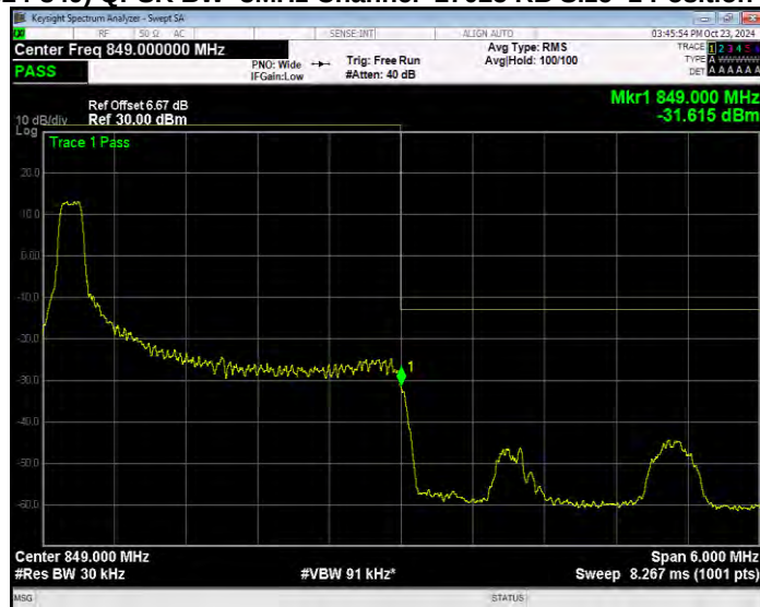
Band26(824-849) QPSK BW=3MHz Channel=27025 RB Size=1 Position=#Max Extended
