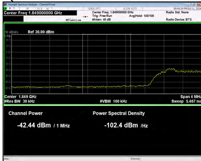
Band25 16QAM BW=5MHz Channel=26065 RB Size=1 Position=#Max Normal
