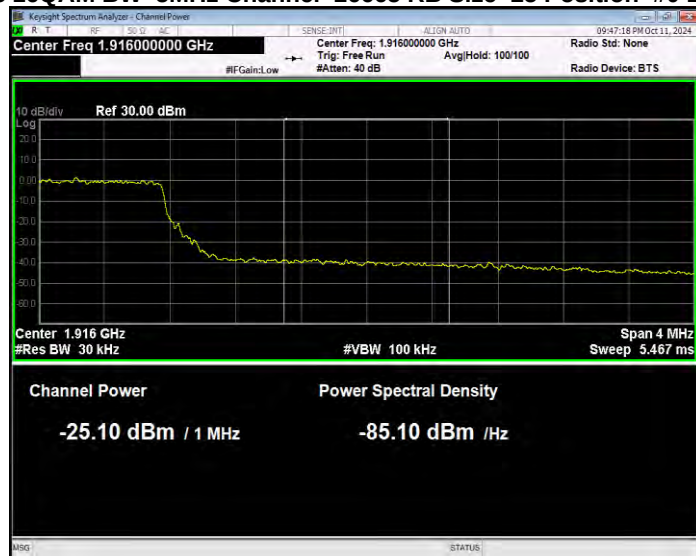
Band25 16QAM BW=5MHz Channel=26665 RB Size=25 Position=#0 Normal
