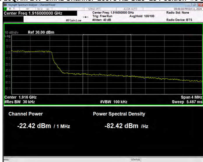
Band25 16QAM BW=3MHz Channel=26675 RB Size=15 Position=#0 Normal
