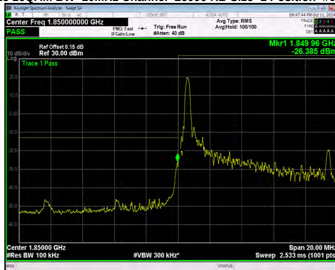
Band25 16QAM BW=10MHz Channel=26090 RB Size=1 Position=#Max Extended
