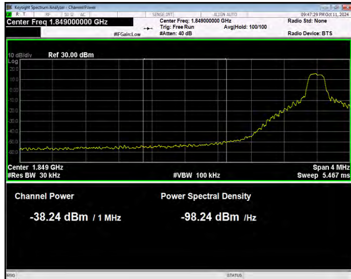
Band25 QPSK BW=10MHz Channel=26090 RB Size=1 Position=#0 Normal
