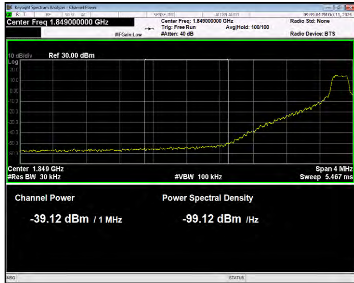
Band25 16QAM BW=15MHz Channel=26115 RB Size=1 Position=#0 Normal
