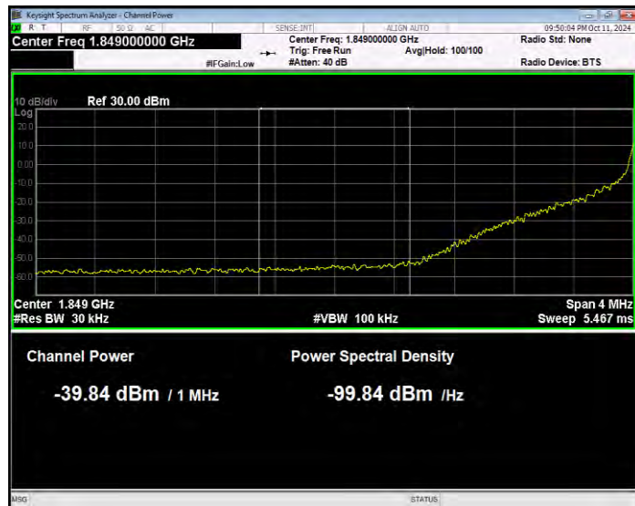
Band25 QPSK BW=20MHz Channel=26140 RB Size=1 Position=#0 Normal
