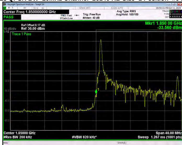
Band25 QPSK BW=20MHz Channel=26140 RB Size=1 Position=#Max Extended
