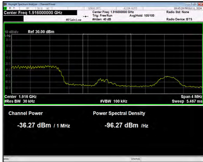
Band25 QPSK BW=3MHz Channel=26675 RB Size=1 Position=#0 Normal
