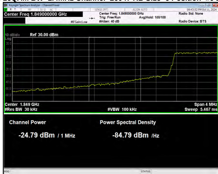
Band25 16QAM BW=1.4MHz Channel=26047 RB Size=6 Position=#0 Normal
