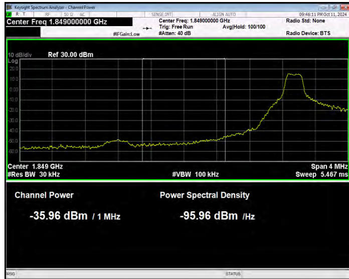
Band25 QPSK BW=5MHz Channel=26065 RB Size=1 Position=#0 Normal
