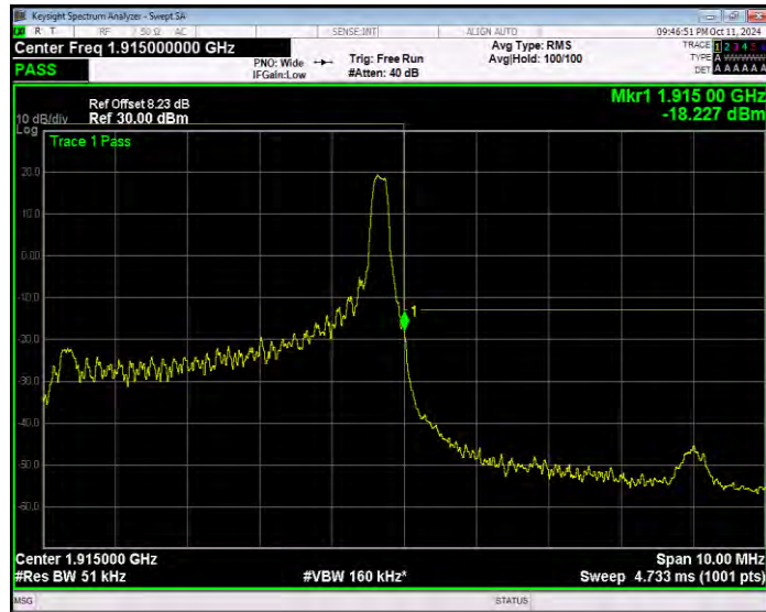
Band25 QPSK BW=5MHz Channel=26665 RB Size=25 Position=#0 Extended
