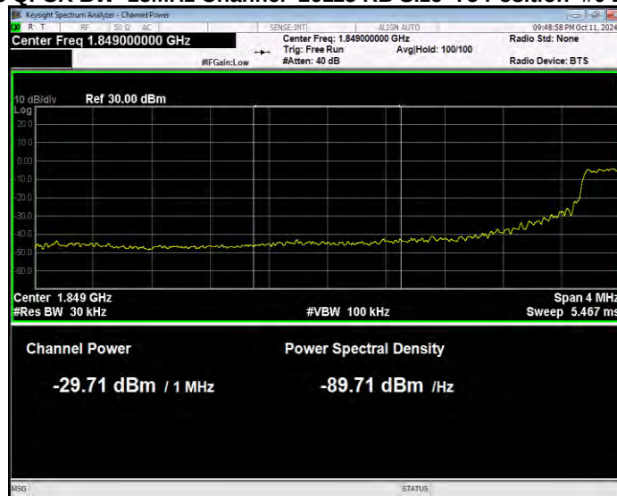
Band25 QPSK BW=15MHz Channel=26115 RB Size=75 Position=#0 Normal
