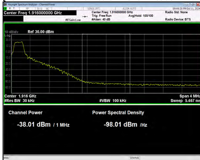
Band25 QPSK BW=15MHz Channel=26615 RB Size=1 Position=#Max Normal
