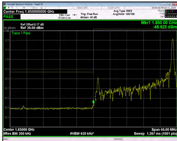
Band25 QPSK BW=20MHz Channel=26140 RB Size=100 Position=#0 Extended
