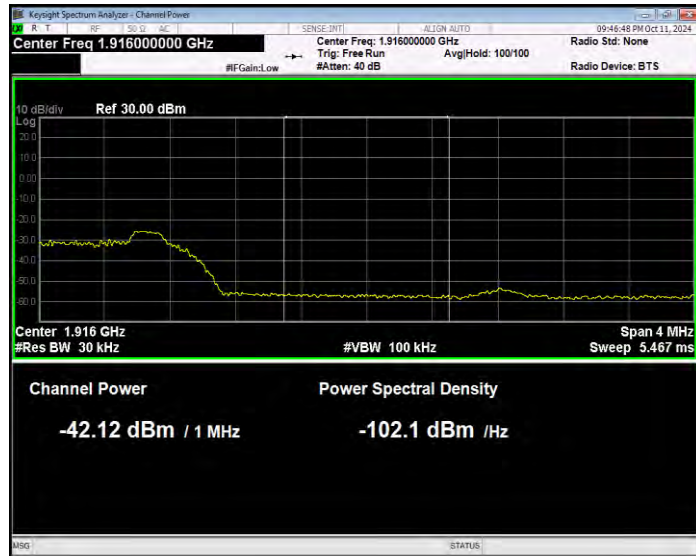
Band25 QPSK BW=5MHz Channel=26665 RB Size=1 Position=#0 Normal
