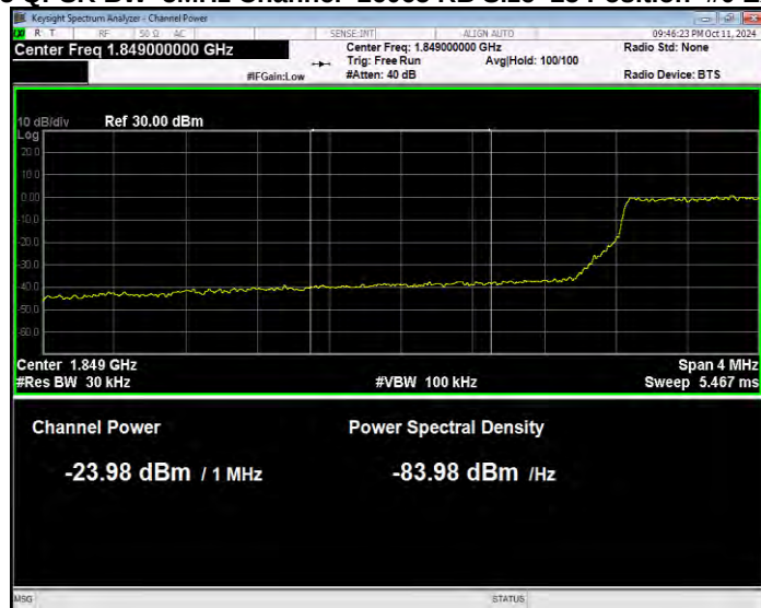
Band25 QPSK BW=5MHz Channel=26065 RB Size=25 Position=#0 Normal
