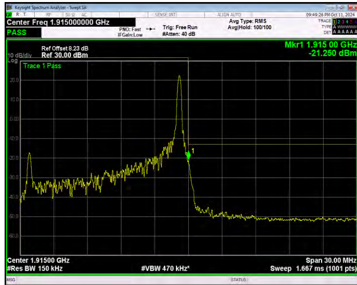
Band25 QPSK BW=15MHz Channel=26615 RB Size=75 Position=#0 Extended
