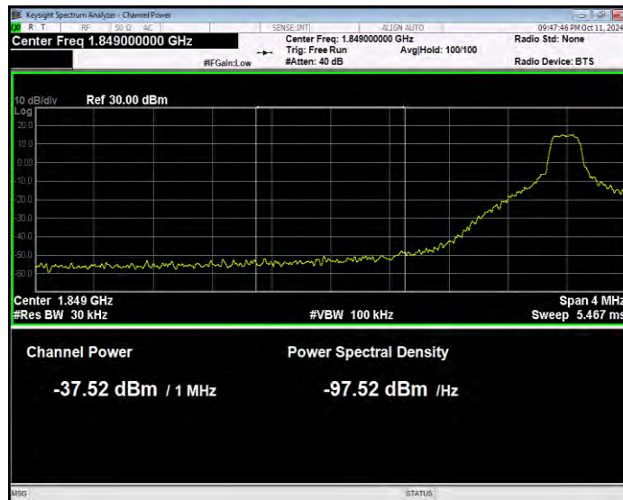
Band25 16QAM BW=10MHz Channel=26090 RB Size=1 Position=#0 Normal
