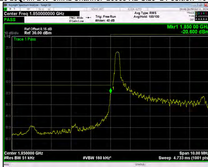
Band25 16QAM BW=5MHz Channel=26065 RB Size=1 Position=#Max Extended
