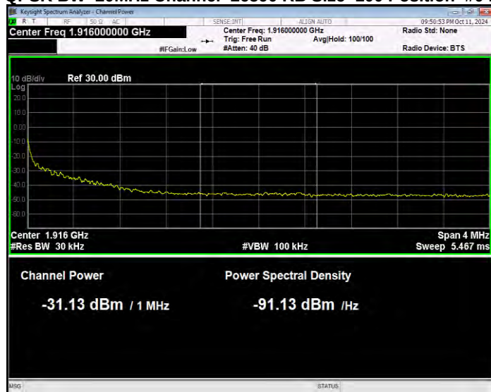
Band25 QPSK BW=20MHz Channel=26590 RB Size=100 Position=#0 Normal
