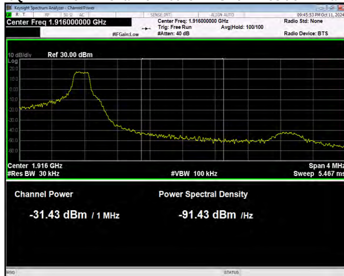
Band25 16QAM BW=3MHz Channel=26675 RB Size=1 Position=#Max Normal
