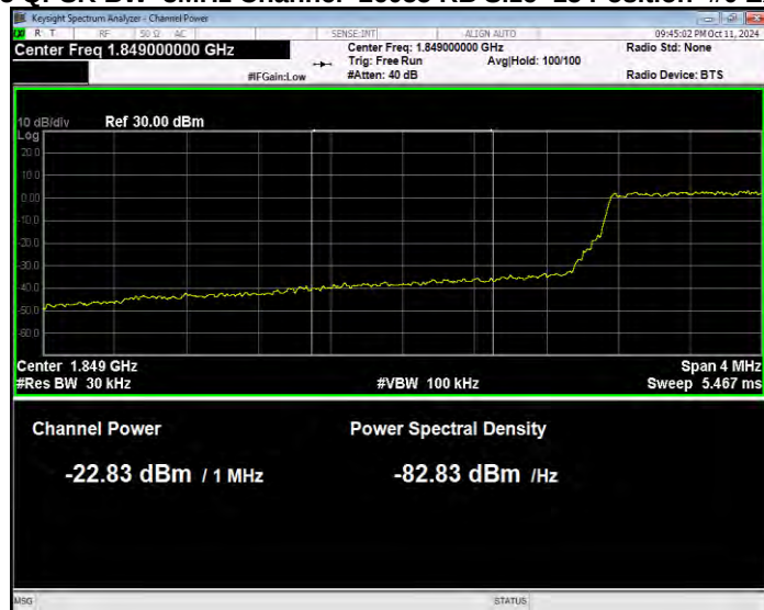
Band25 QPSK BW=3MHz Channel=26055 RB Size=15 Position=#0 Normal
