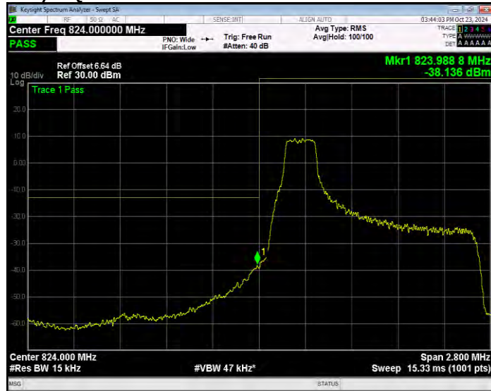
Band26(824-849) 16QAM BW=1.4MHz Channel=26797 RB Size=1 Position=#Max Extended
