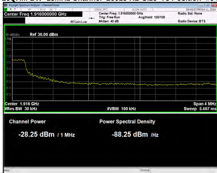
Band25 16QAM BW=15MHz Channel=26615 RB Size=75 Position=#0 Normal
