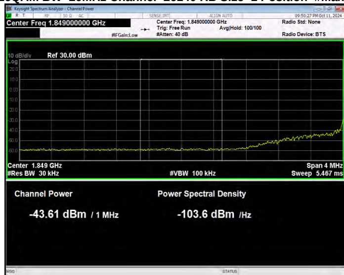
Band25 16QAM BW=20MHz Channel=26140 RB Size=1 Position=#Max Normal
