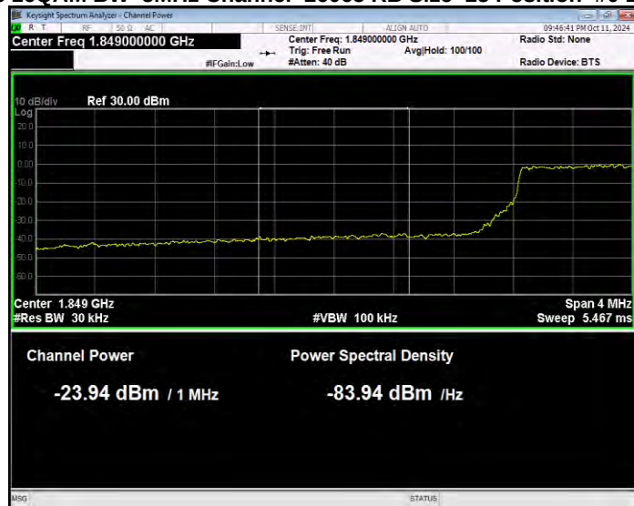
Band25 16QAM BW=5MHz Channel=26065 RB Size=25 Position=#0 Normal
