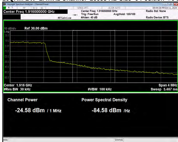
Band25 16QAM BW=1.4MHz Channel=26683 RB Size=6 Position=#0 Normal
