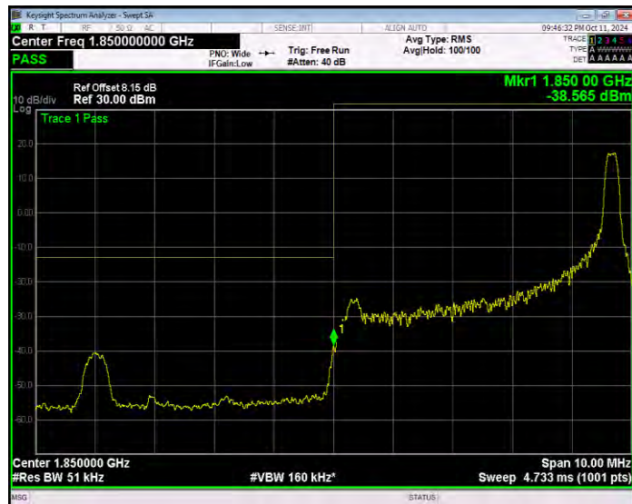
Band25 16QAM BW=5MHz Channel=26065 RB Size=25 Position=#0 Extended
