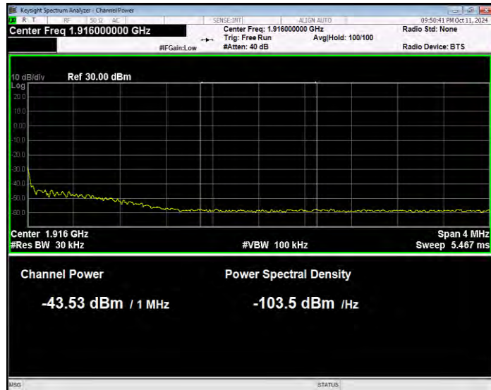
Band25 QPSK BW=20MHz Channel=26590 RB Size=1 Position=#0 Normal
