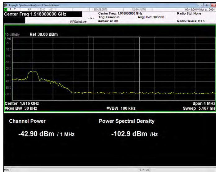
Band25 QPSK BW=10MHz Channel=26640 RB Size=1 Position=#0 Normal
