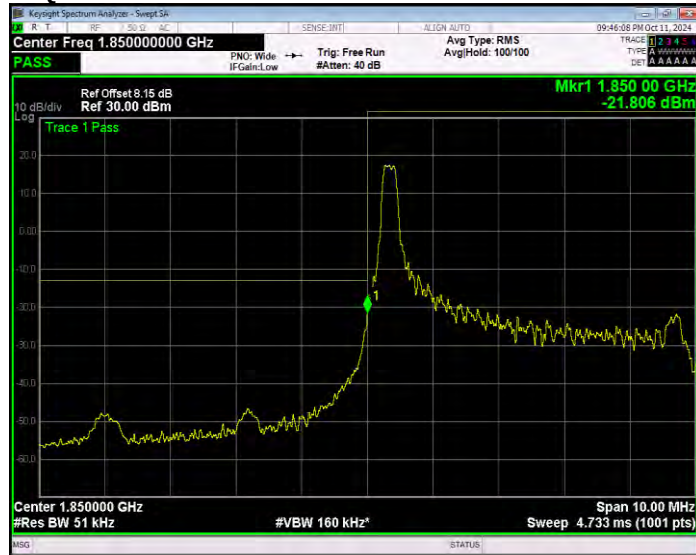
Band25 QPSK BW=5MHz Channel=26065 RB Size=1 Position=#Max Extended
