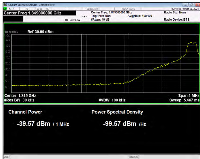
Band25 QPSK BW=15MHz Channel=26115 RB Size=1 Position=#0 Normal
