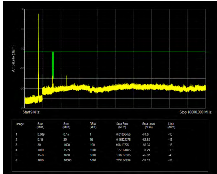
Band13 QPSK BW=5MHz Channel=23205 RB Size=1 Position=#0
