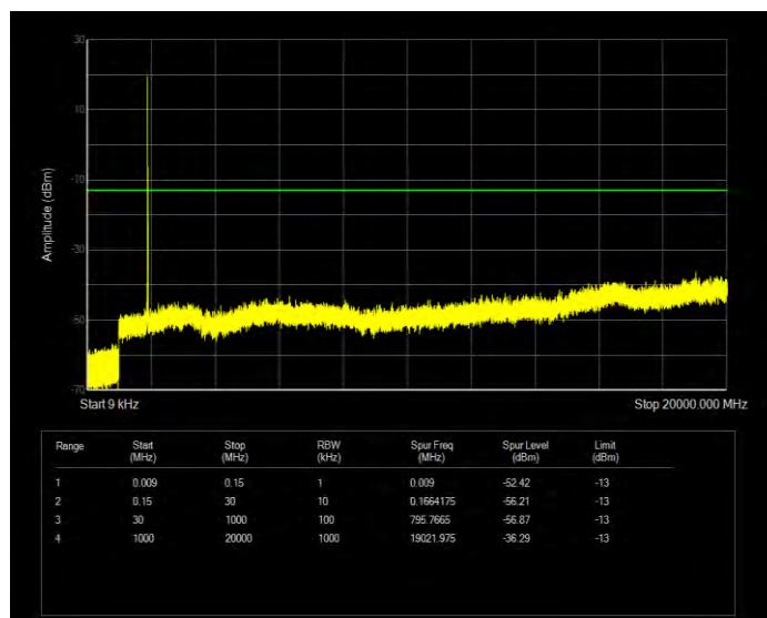
Band25 QPSK BW=20MHz Channel=26140 RB Size=1 Position=#0
