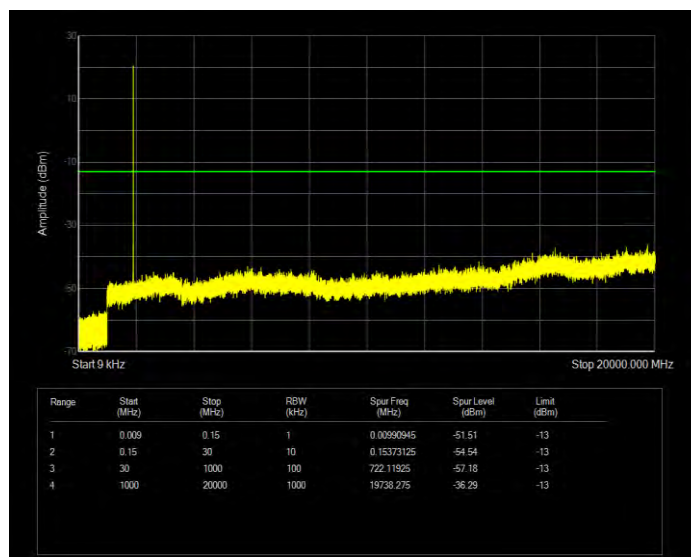
Band25 16QAM BW=10MHz Channel=26090 RB Size=1 Position=#0
