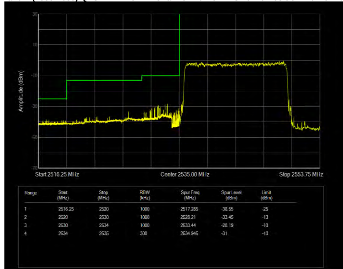
Band41(2535-2655) QPSK BW=15MHz Channel=41165 RB Size=1 Position=#0 Extended
