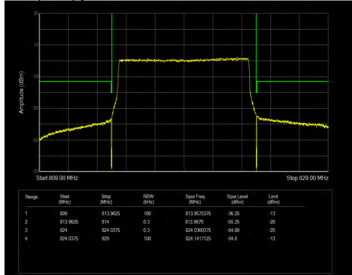
Band26(814-824) QPSK BW=3MHz Channel=26705 RB Size=1 Position=#0 Extended
