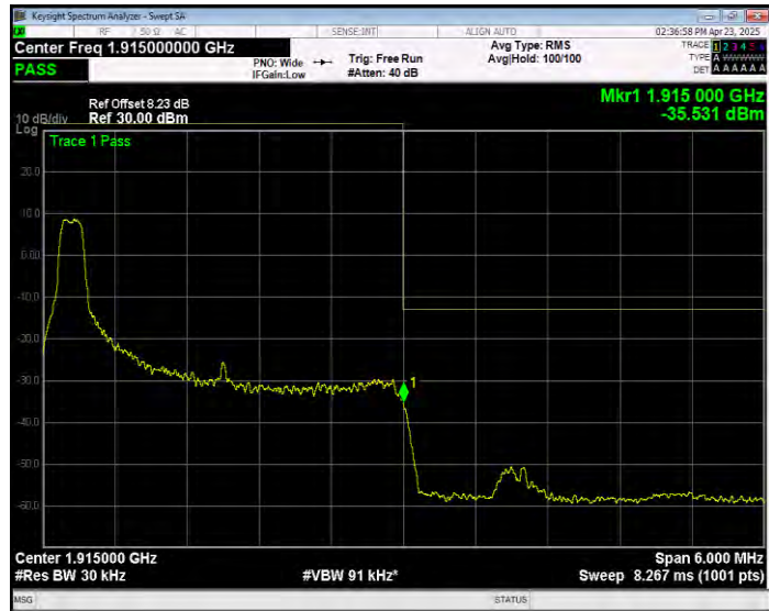
Band25 QPSK BW=3MHz Channel=26675 RB Size=1 Position=#Max Extended
