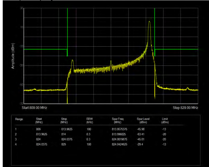
Band26(814-824) 16QAM BW=10MHz Channel=26740 RB Size=50 Position=#0 Extended
