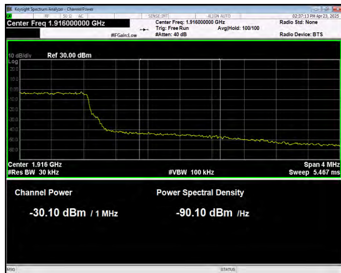
Band25 QPSK BW=3MHz Channel=26675 RB Size=15 Position=#0 Normal
