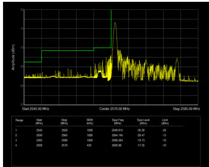
Band38 16QAM BW=20MHz Channel=37850 RB Size=1 Position=#Max Extended
