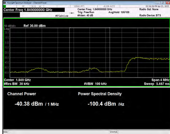
Band25 QPSK BW=3MHz Channel=26055 RB Size=1 Position=#Max Normal
