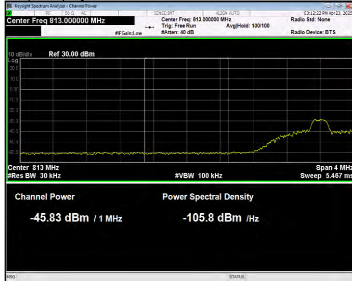
Band26(814-824) 16QAM BW=10MHz Channel=26740 RB Size=1 Position=#Max Normal
