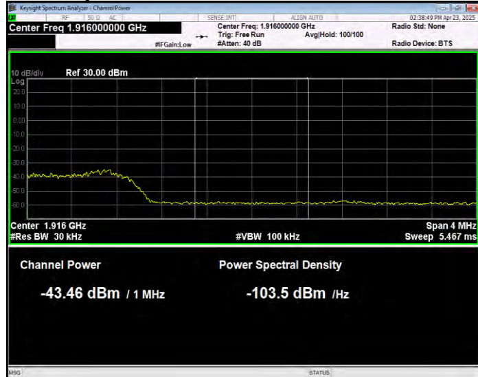
Band25 QPSK BW=5MHz Channel=26665 RB Size=1 Position=#0 Normal
