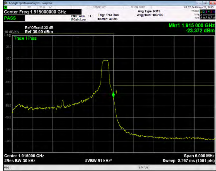
Band25 QPSK BW=3MHz Channel=26675 RB Size=15 Position=#0 Extended
