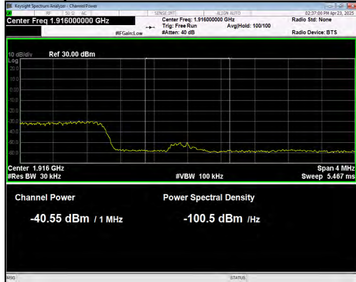
Band25 QPSK BW=3MHz Channel=26675 RB Size=1 Position=#0 Normal
