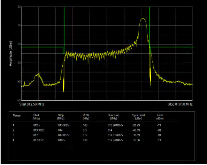
Band26(814-824) 16QAM BW=3MHz Channel=26705 RB Size=15 Position=#0 Extended
