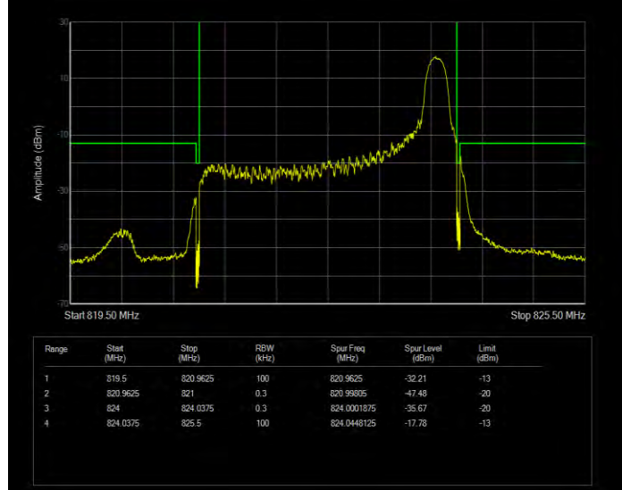
Band26(814-824) QPSK BW=3MHz Channel=26775 RB Size=15 Position=#0 Extended
