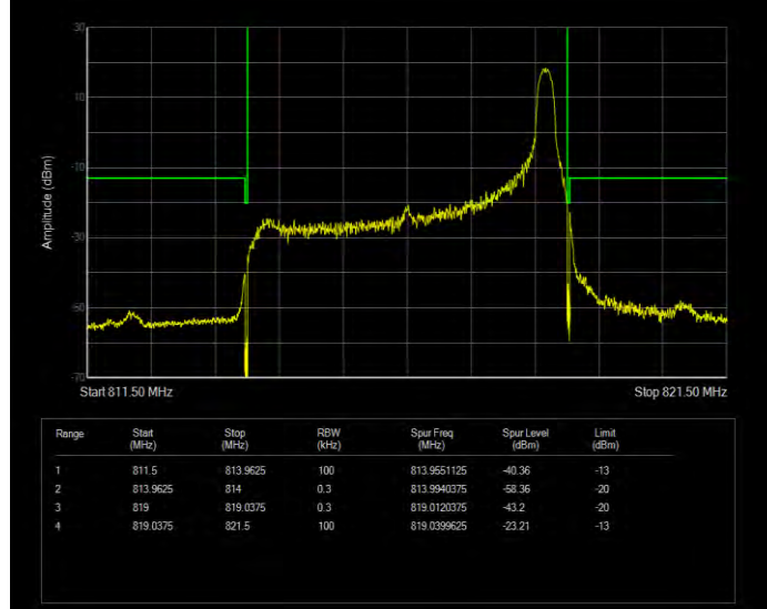
Band26(814-824) QPSK BW=5MHz Channel=26715 RB Size=25 Position=#0 Extended
