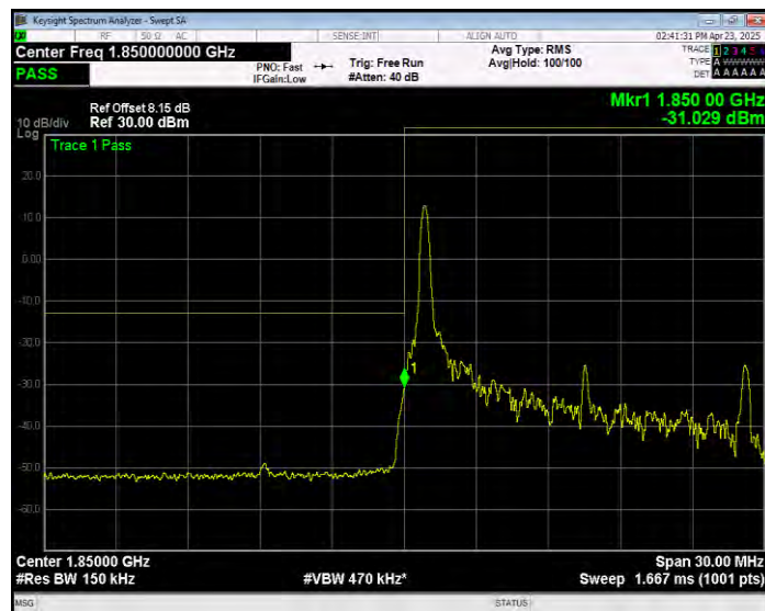
Band25 16QAM BW=15MHz Channel=26115 RB Size=1 Position=#Max Extended
