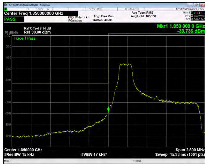
Band25 QPSK BW=1.4MHz Channel=26047 RB Size=1 Position=#Max Extended
