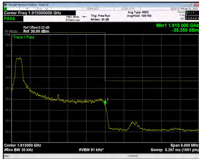
Band25 16QAM BW=3MHz Channel=26675 RB Size=1 Position=#Max Extended
