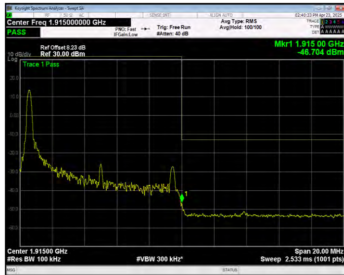
Band25 QPSK BW=10MHz Channel=26640 RB Size=1 Position=#Max Extended
