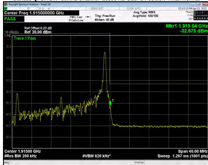
Band25 QPSK BW=20MHz Channel=26590 RB Size=100 Position=#0 Extended
