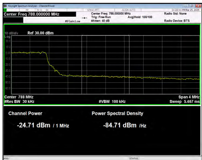
Band13 QPSK BW=5MHz Channel=23255 RB Size=25 Position=#0 Normal
