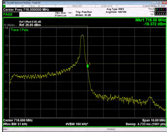
Band17 QPSK BW=5MHz Channel=23825 RB Size=25 Position=#0 Extended
