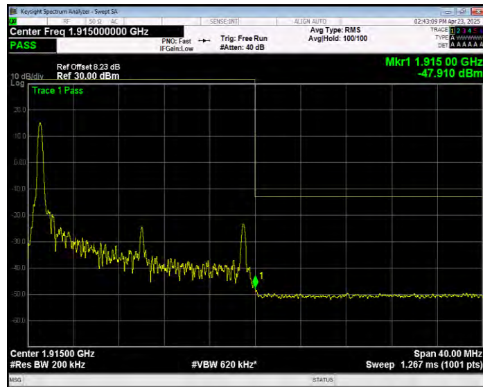
Band25 QPSK BW=20MHz Channel=26590 RB Size=1 Position=#Max Extended
