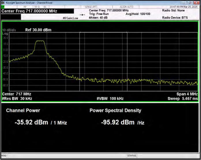
Band12 16QAM BW=5MHz Channel=23155 RB Size=1 Position=#Max Normal
