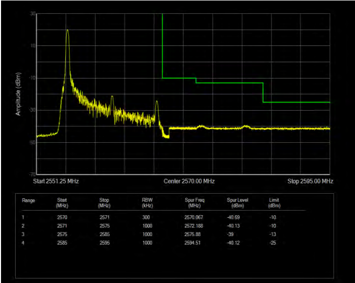
Band7 QPSK BW=15MHz Channel=21375 RB Size=1 Position=#Max Extended
