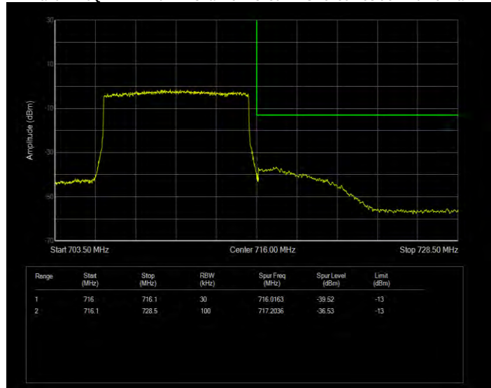
Band12 16QAM BW=3MHz Channel=23025 RB Size=1 Position=#0 Extended
