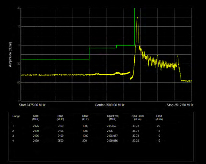
Band7 QPSK BW=10MHz Channel=20800 RB Size=1 Position=#Max Extended
