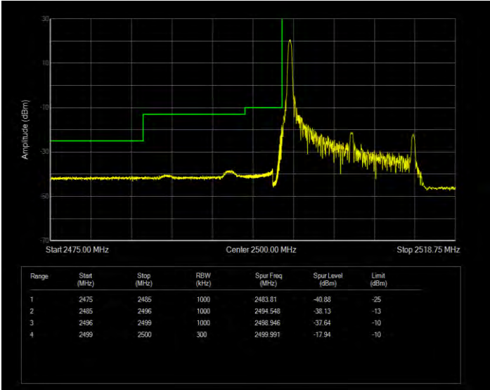
Band7 QPSK BW=15MHz Channel=20825 RB Size=1 Position=#Max Extended
