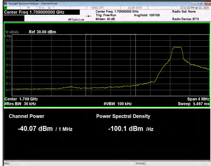
Band4 QPSK BW=5MHz Channel=19975 RB Size=1 Position=#0 Normal
