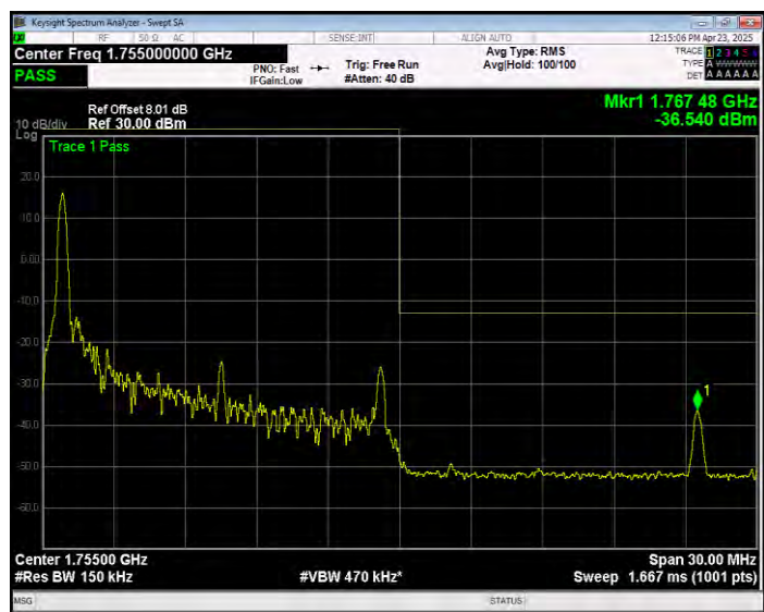
Band4 QPSK BW=15MHz Channel=20325 RB Size=1 Position=#Max Extended
