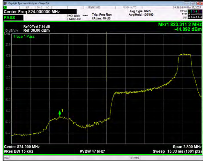
Band5 QPSK BW=1.4MHz Channel=20407 RB Size=6 Position=#0 Extended
