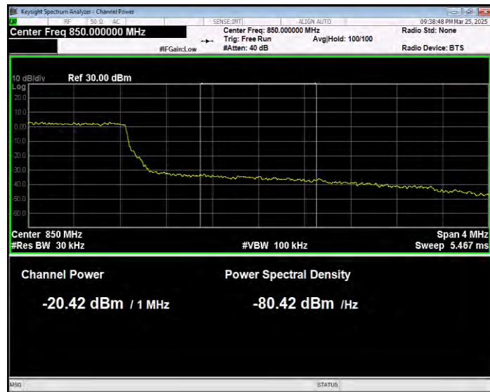
Band5 16QAM BW=3MHz Channel=20635 RB Size=15 Position=#0 Normal
