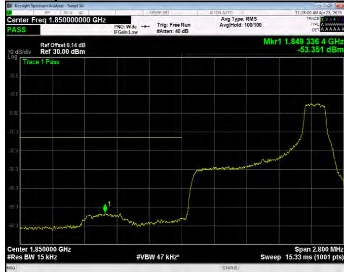
Band2 QPSK BW=1.4MHz Channel=18607 RB Size=6 Position=#0 Extended
