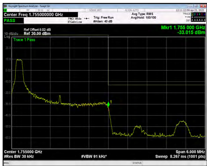
Band4 16QAM BW=3MHz Channel=20385 RB Size=1 Position=#Max Extended
