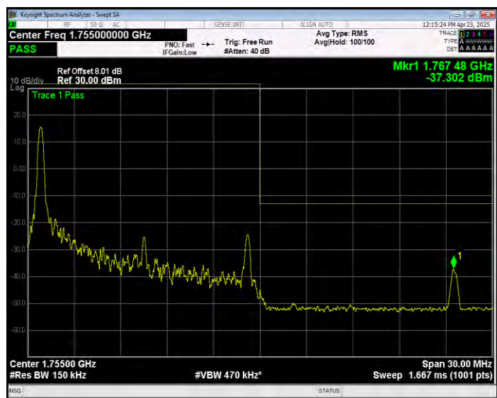
Band4 16QAM BW=15MHz Channel=20325 RB Size=1 Position=#Max Extended
