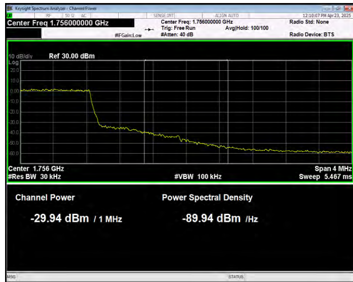
Band4 16QAM BW=1.4MHz Channel=20393 RB Size=6 Position=#0 Normal
