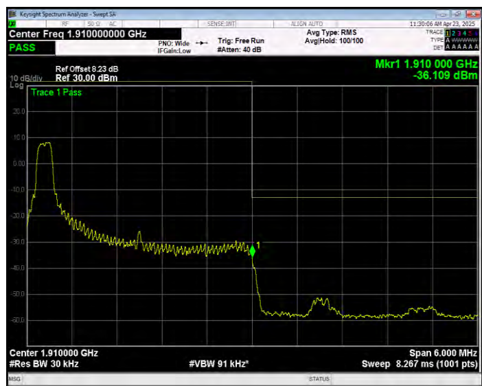
Band2 QPSK BW=3MHz Channel=19185 RB Size=1 Position=#Max Extended
