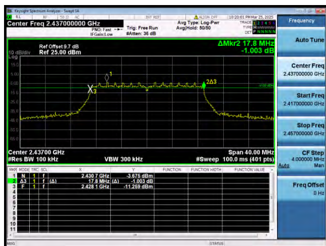
802.11n_Band2.4G_BW20MHz MHz
