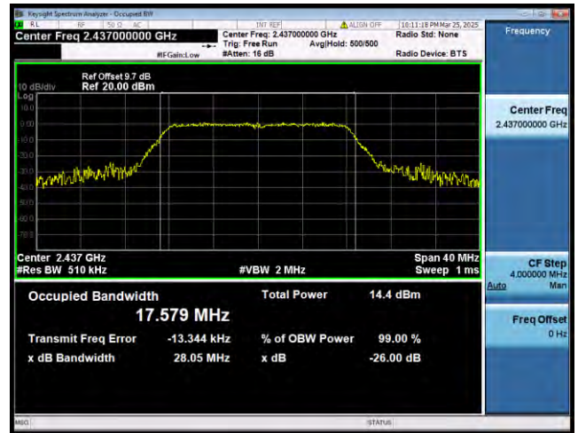
802.11g MHz
