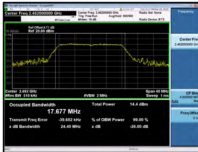
802.11g MHz
