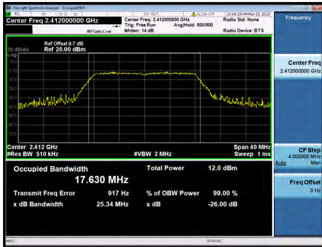
802.11g MHz
