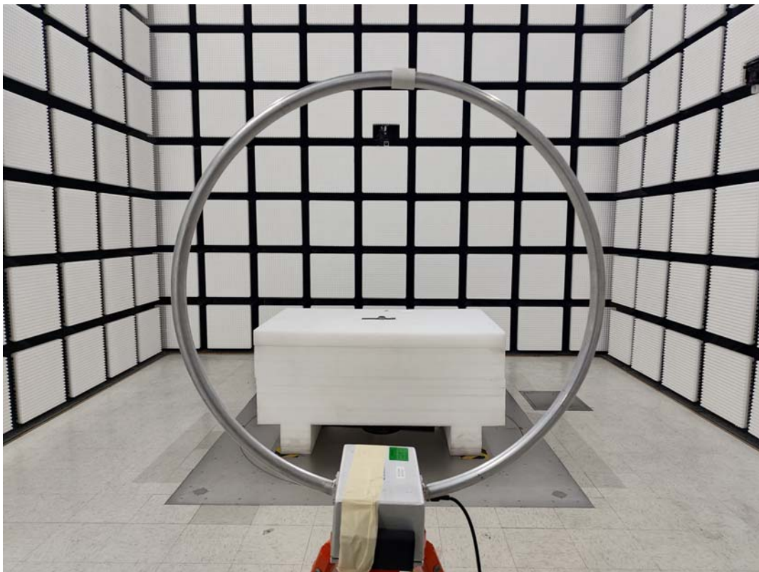
Radiated Emission 9kHz-30MHz View-Parallel
