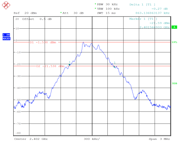
GFSK_Low 0.863 MHz
