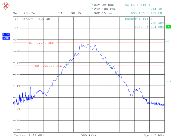
GFSK_High 0.893 MHz
