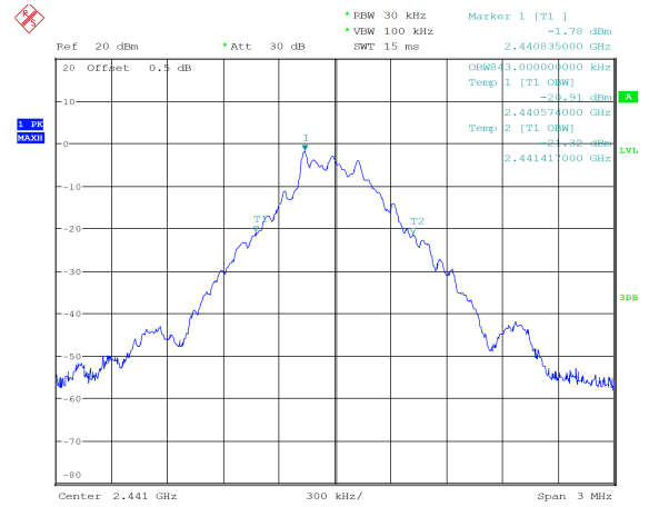
GFSK_Middle 0.843 MHz
