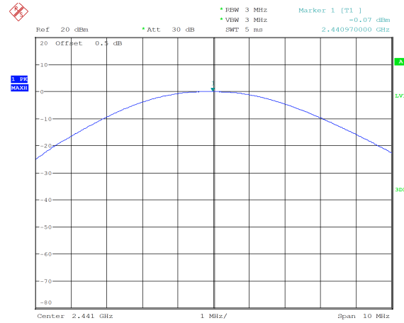
GFSK_Middle -0.07 dBm
