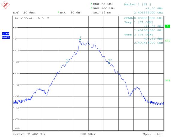
GFSK_Low 0.840 MHz
