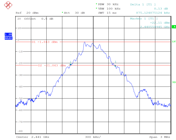
GFSK_Middle 0.875 MHz
