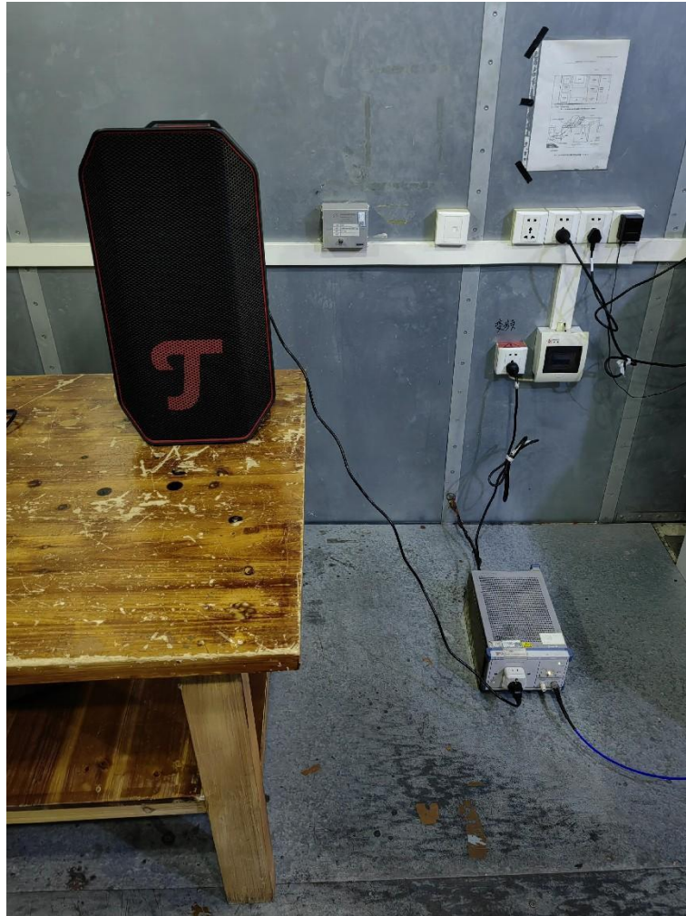
Conducted Emissions at Mains Terminals 150 kHz to 30 MHz
