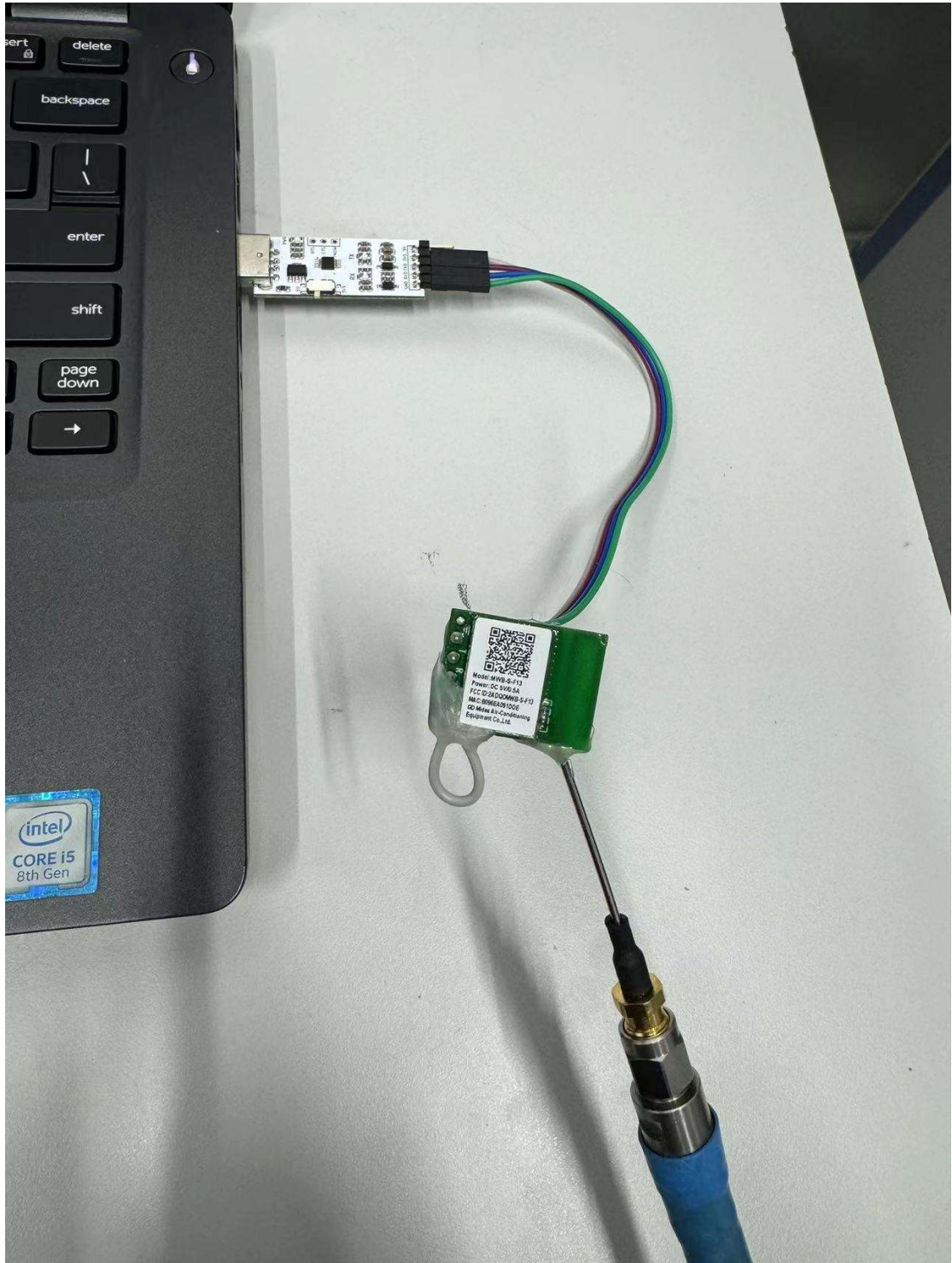
RF test (Conducted)
