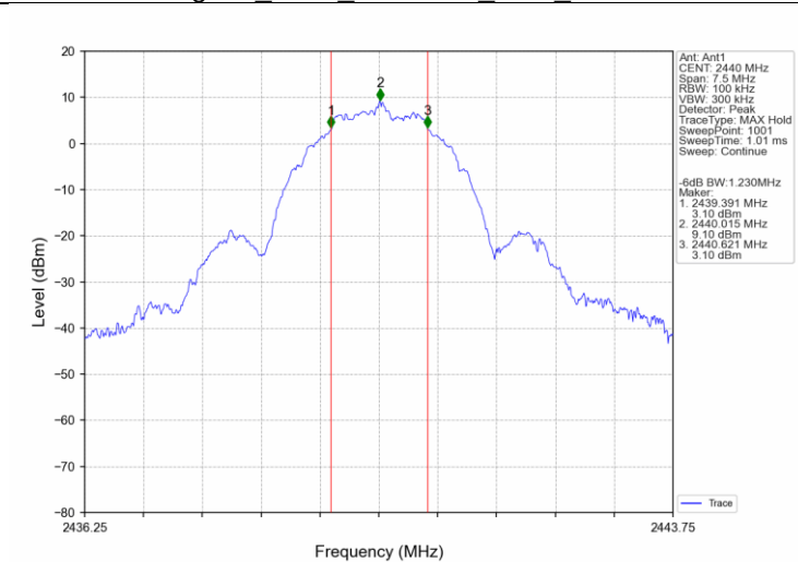
Zigbee_MCH_2440MHz_Ant1_NTNV
