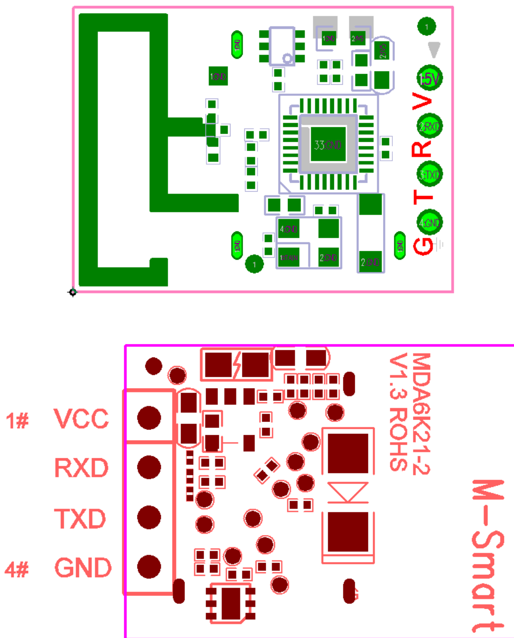
Figure 2.1 Terminal Interface
