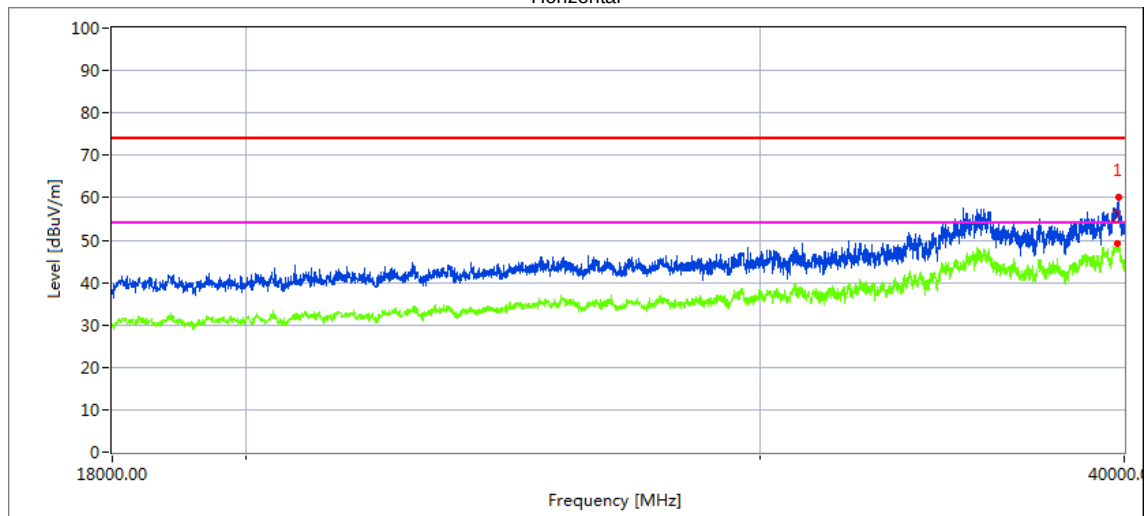
Low Channel (5180 MHz)-Above 1G Horizontal
