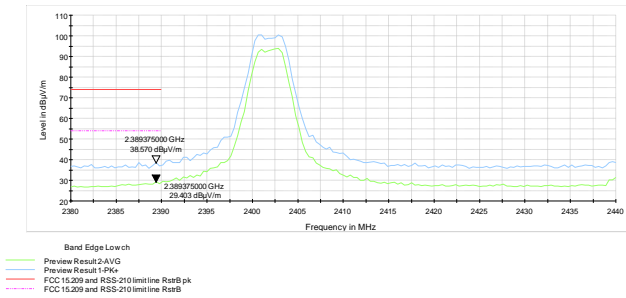
Figure 7.6-3: Band edge spurious emissions at 2390 MHz
