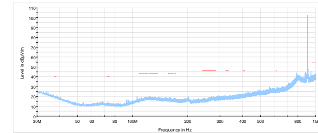
Figure 7.6-8: Radiated spurious emissions on below 1 GHz, Low ch.
