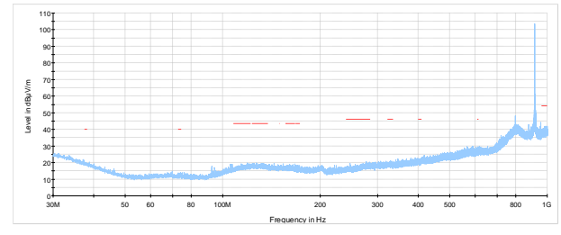
Figure 7.6-9: Radiated spurious emissions on below 1 GHz, Mid ch.
