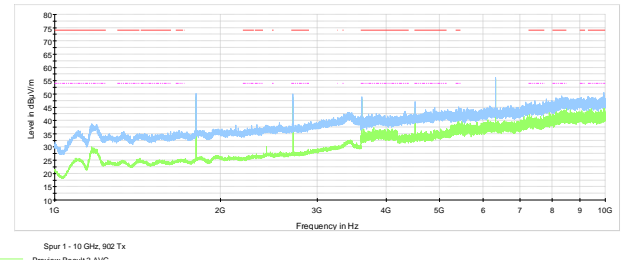
Figure 7.6-11: Radiated spurious emissions on above 1 GHz, Low ch.
