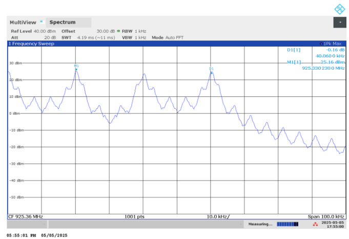
Figure 7.4-8: Carrier frequency separation
