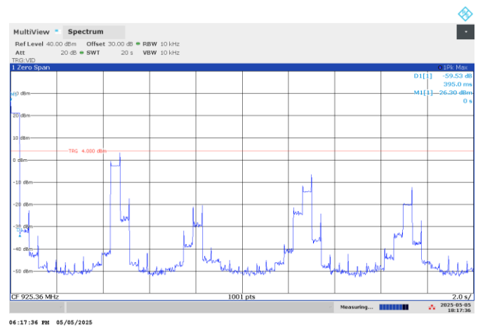
Figure 7.4-10: Dwell time, in sweep time 20s
