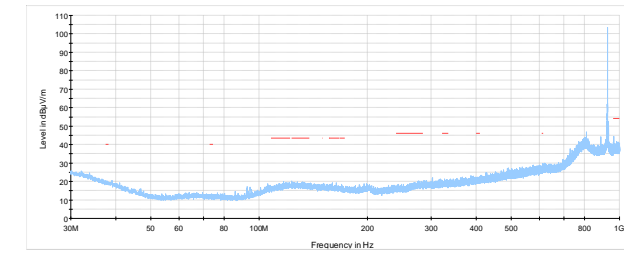
Figure 7.6-10: Radiated spurious emissions on below 1 GHz, High ch.
