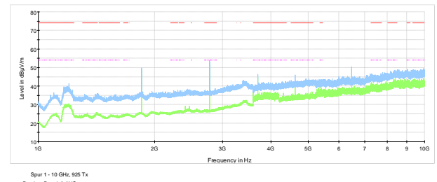
Figure 7.6-13: Radiated spurious emissions on above 1 GHz, High ch.
