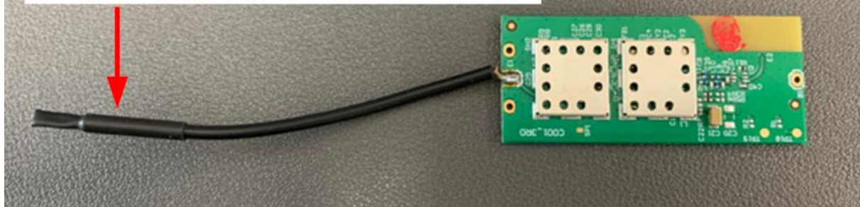
FHSS Antenna (Tx and Rx) 903.28 MHz - 925.36 MHz
