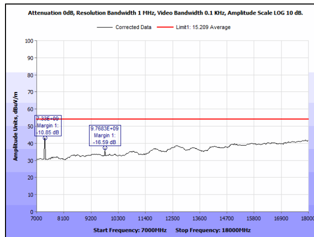
Plot 16. Radiated Harmonics, Mid Channel, 2440 MHz, 7 GHz – 18 GHz, Average
