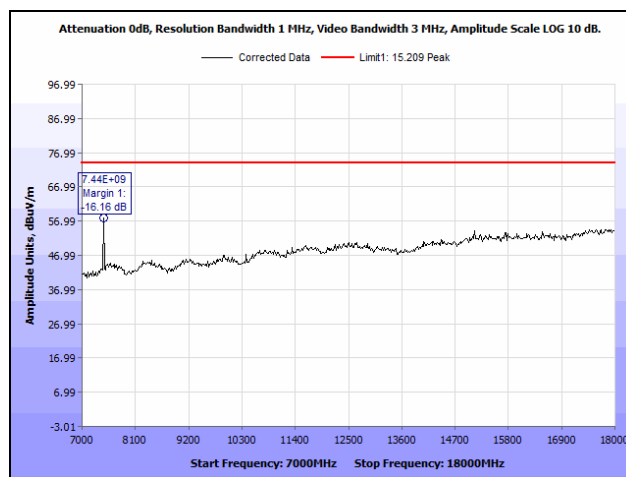
Plot 22. Radiated Harmonics, High Channel, 2481 MHz, 7 GHz – 18 GHz, Peak
