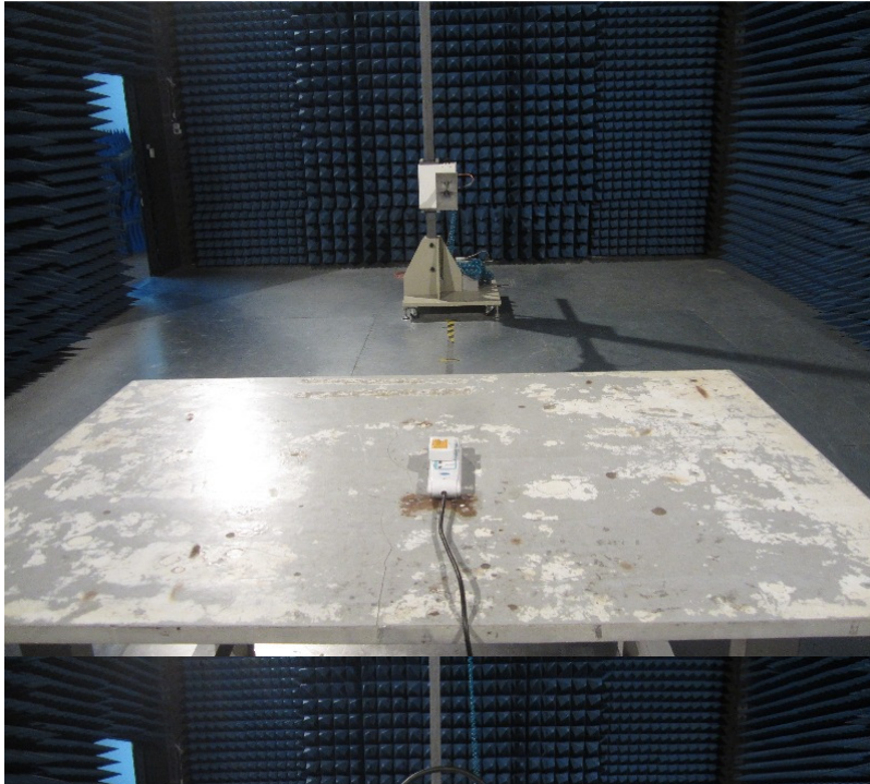
Setup for radiated emission
