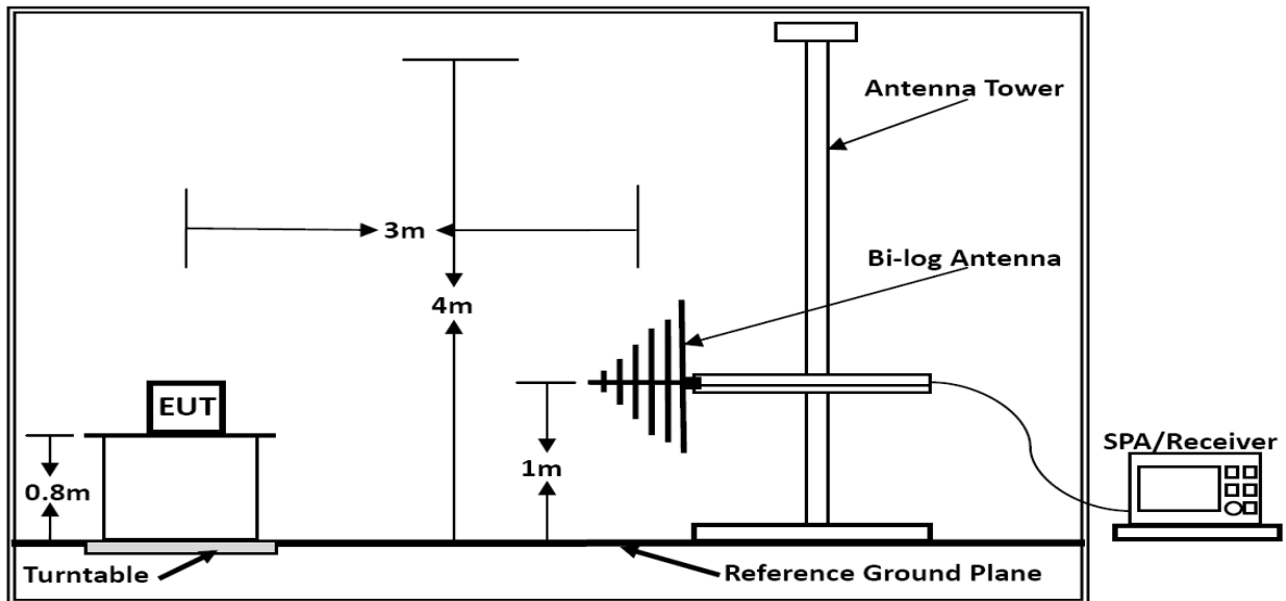
Below 1GHz
