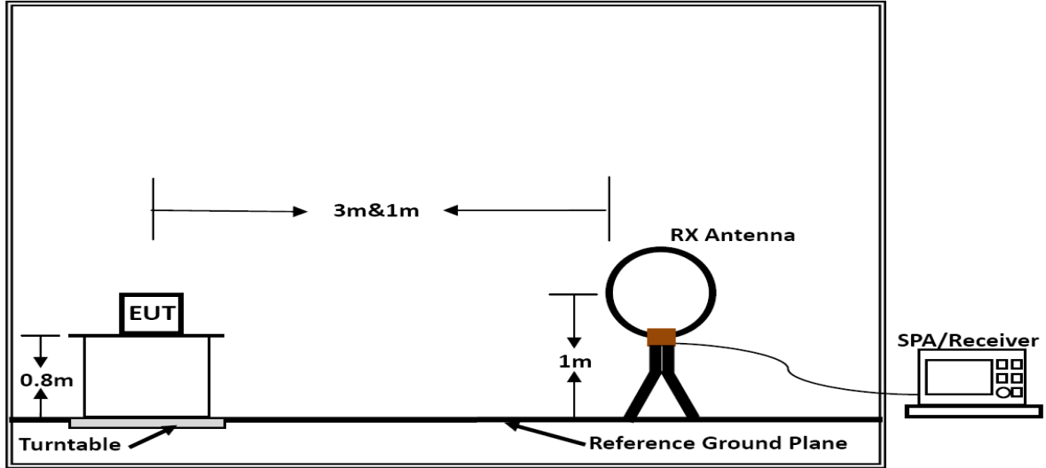
Below 30MHz
