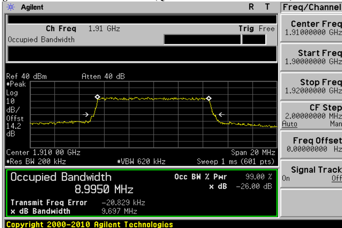
Figure 8-39: 10MHz BW LTE-Band 25(QPSK RB Number: 50 Offset: 0) Channel High
