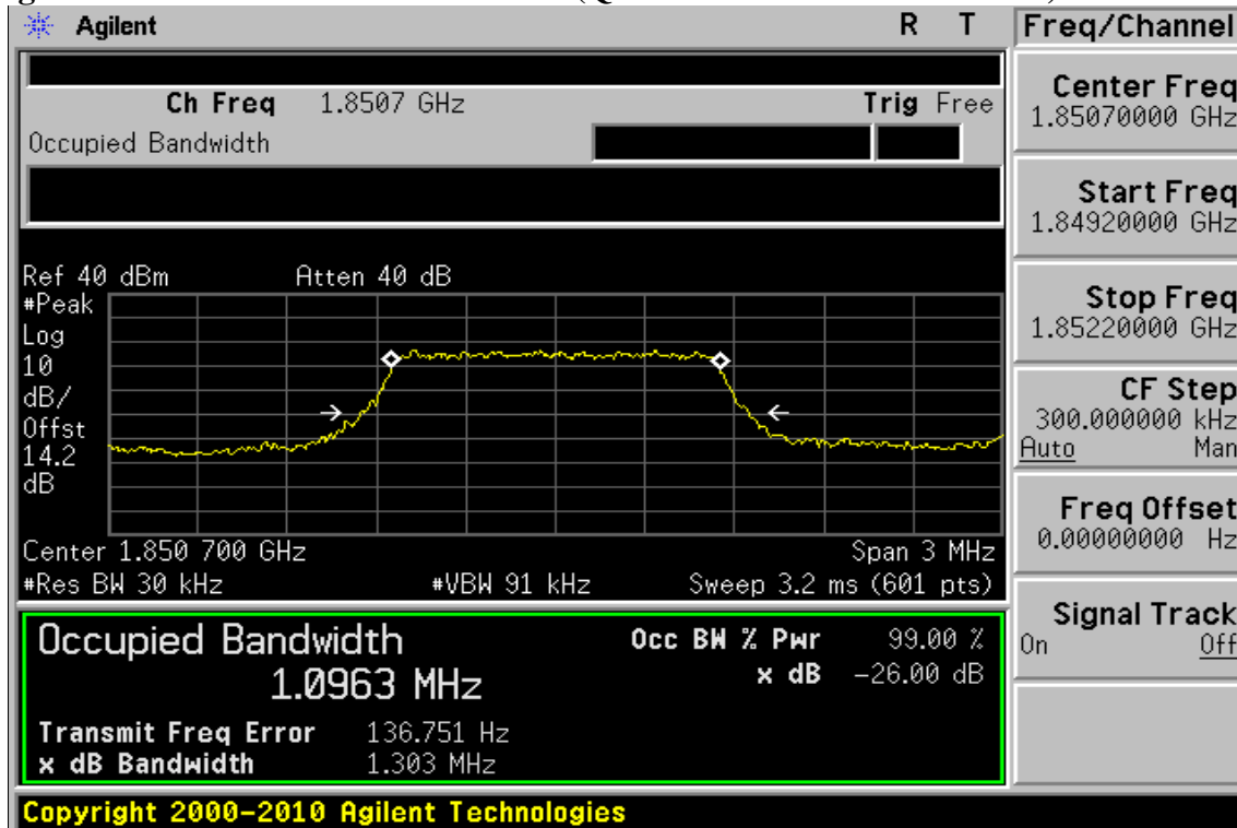
Figure 8-19: 1.4MHz BW LTE-Band 25(QPSK RB Number: 6 Offset: 0) Channel Low
