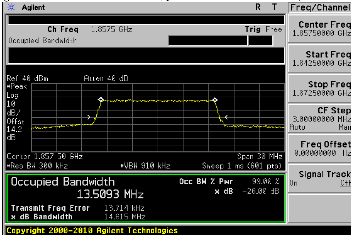
Figure 8-43: 15MHz BW LTE-Band 25(QPSK RB Number: 75 Offset: 0) Channel Low
