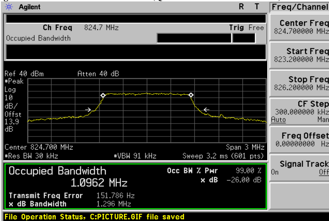
Figure 8-55: 1.4MHz BW LTE-Band 26(QPSK RB Number: 6 Offset: 0) Channel Low
