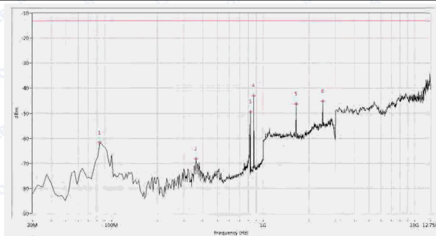
(PlotB.6: GSM 1900MHz Channel = 810, Test Antenna Vertical)
