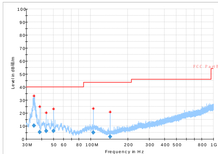
Fig.83 Radiated Spurious Emission (802.11 g,Ch11,30MHz~1GHz)
