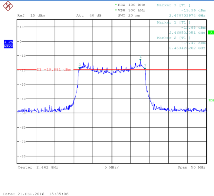
Fig.24 Occupied 6dB Bandwidth (802.11n-20MHz, Ch11)
