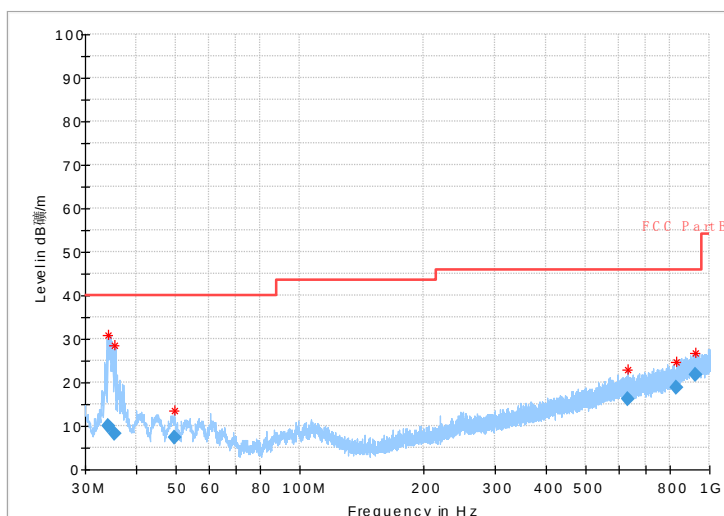
Fig.57 Radiated Spurious Emission (802.11b,Ch11,30MHz~1GHz)
