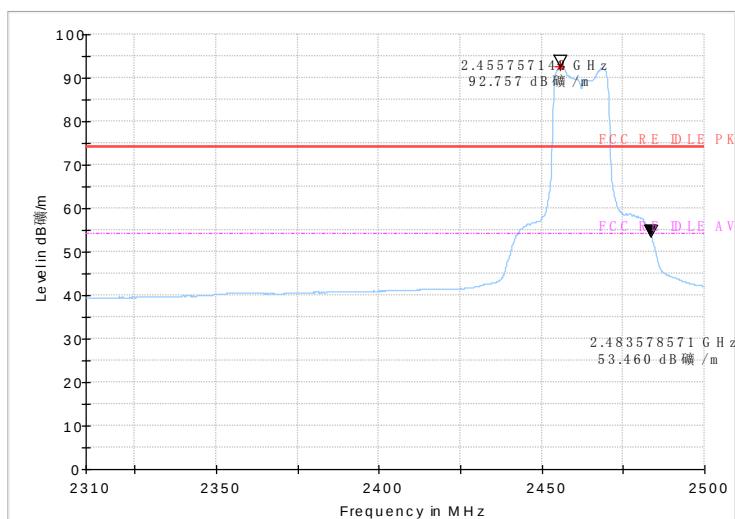
Fig.65 Radiated emission (Power): 802.11g, channel 11
