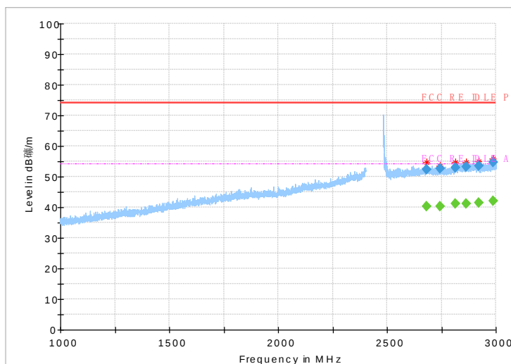
Fig.47 Radiated emission: 8DPSK, Ch78, 1GHz~3GHz
