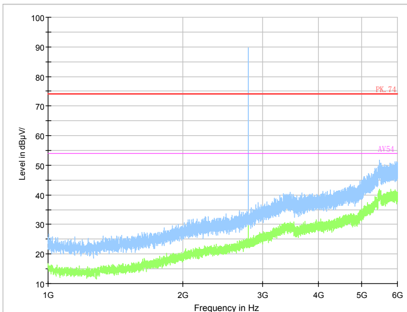
Frequency Range: 1GHz-6GHz Detector: Av mode and PK mode Modulation type: GFSK (LE)
