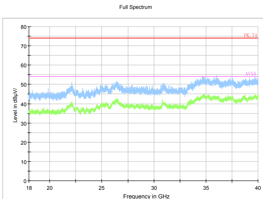
Pic17. Radiated emission (18GHz –40GHz)
