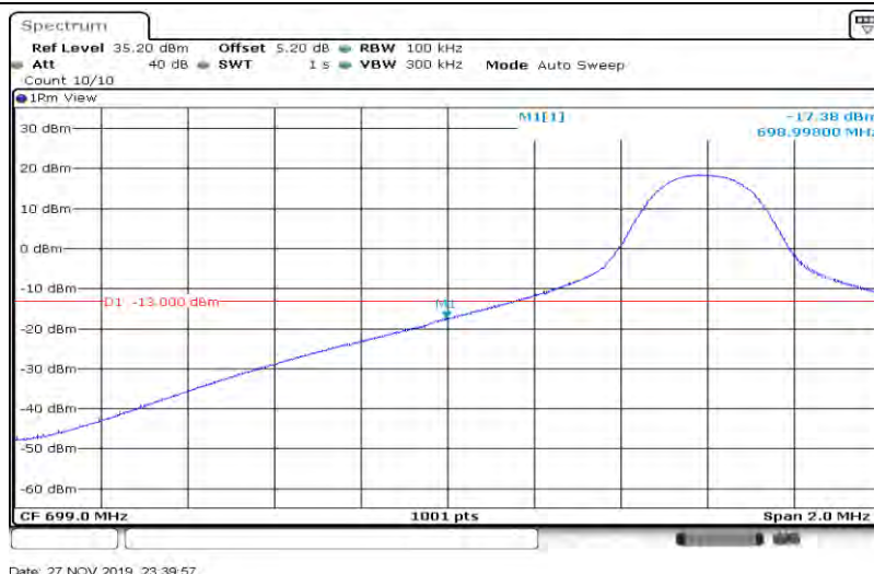
Band12-10MHz-16QAM-23060-50RB#0
