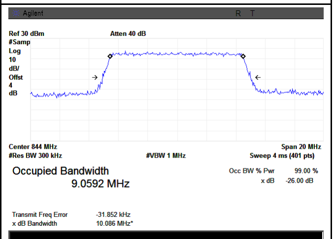
LTE band 5 - High CH 16QAM-10
