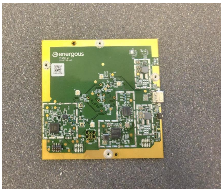
PCB Bottom View with No Shield
